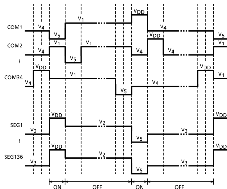
LCD driver timing chart (1/34 duty)
