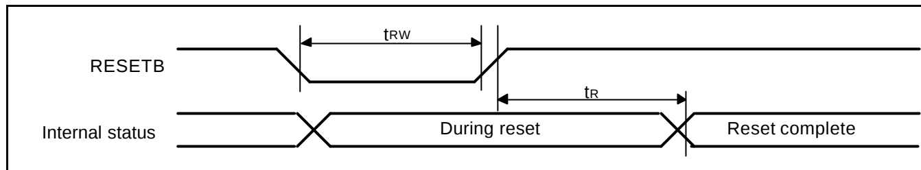
Figure 41. Reset Input Timing Diagram
