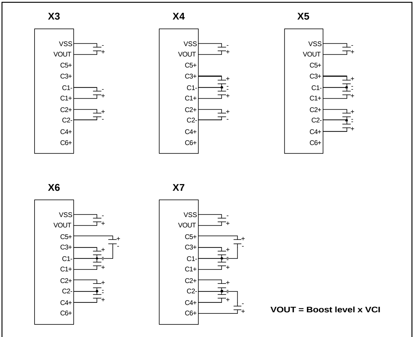
Figure 18. Boosting Circuits
