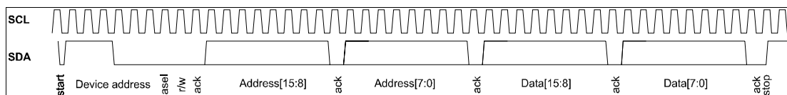
Fig. 6-1: I 2 C_Write timing (in this case NrOfWbytes =5).
