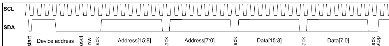
Fig. 2–8: I2C_Write timing (NrOfBytes = 2)
