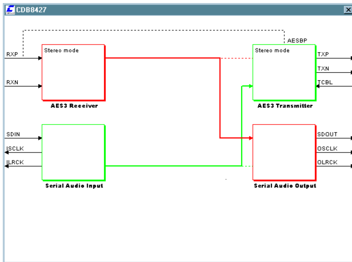
Figure 1. CDB8427 Control Panel Main Window
