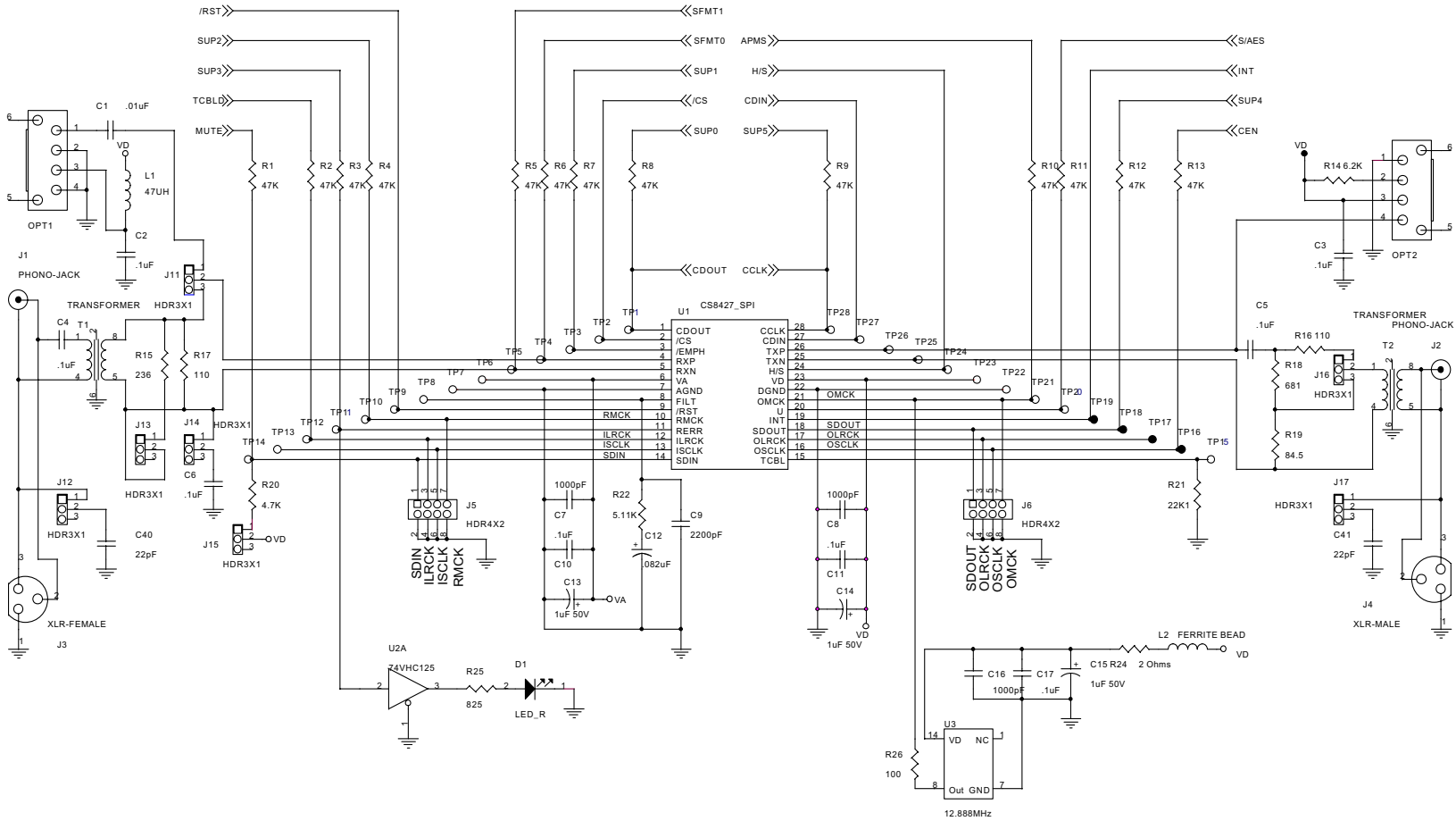
Figure 3. CS8427 Digital Audio Transceiver
