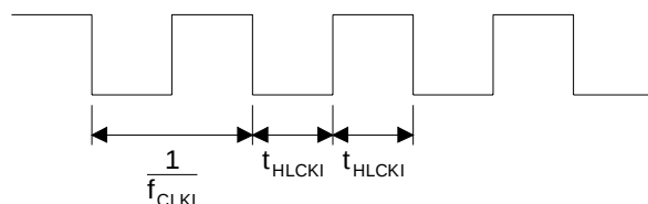
Figure 1. CLKI Timing
