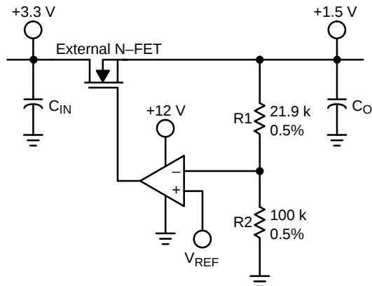
Figure 9. V_{REF} Used in an N-FET LDO Regulator
