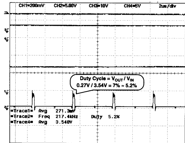
Figure 12. Pulse-By-Pulse Regulation During Soft Start (2.0 \mu s/div)
