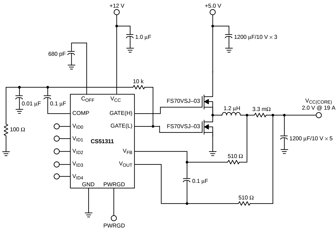
Figure 1. Application Diagram
