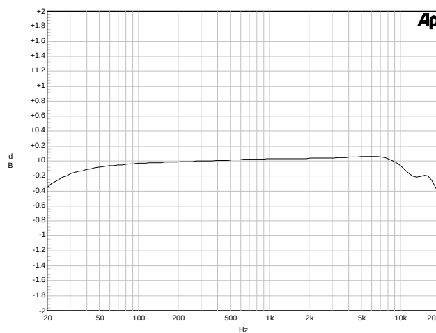
Figure 21. Line Output - Frequency Response at 3.0 V
