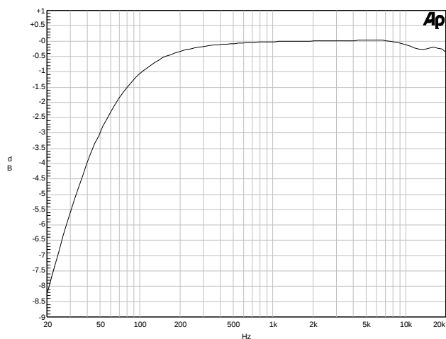
Figure 14. Headphone Output - Frequency Response at 1.8 V
