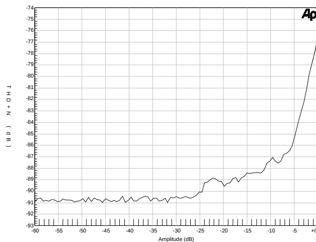
Figure 17. Headphone Output - THD+N versus Amplitude at 3.0 V
