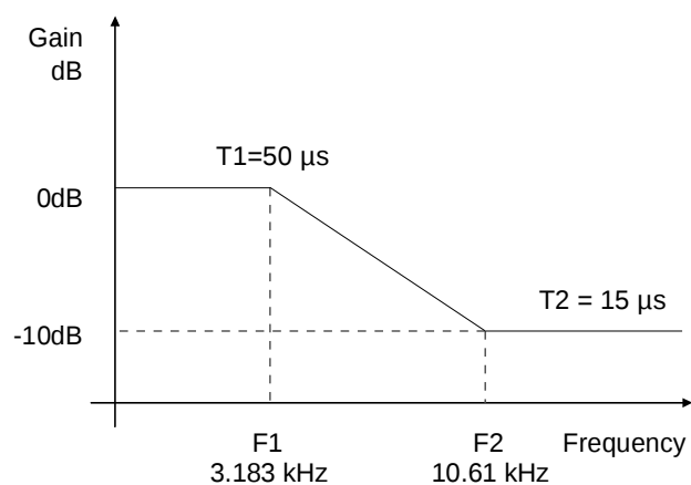
Figure 30. De-Emphasis Curve
