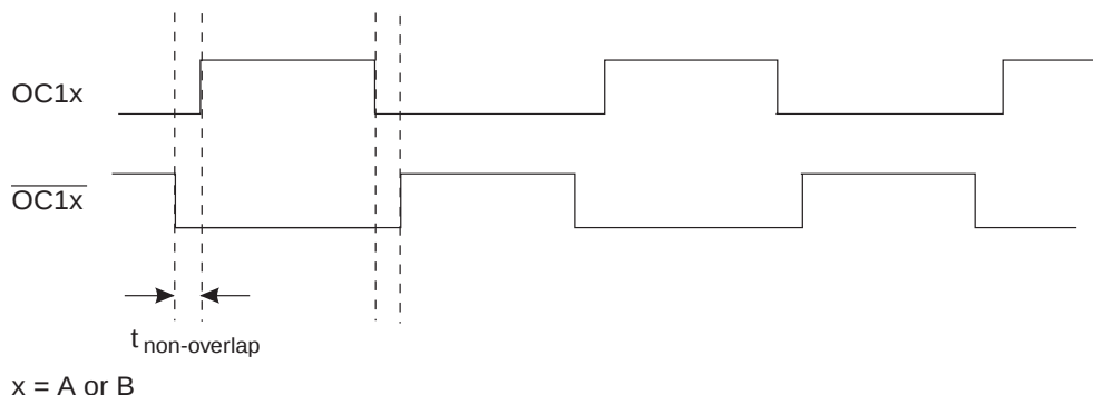
Figure 36. 无重叠输出对
