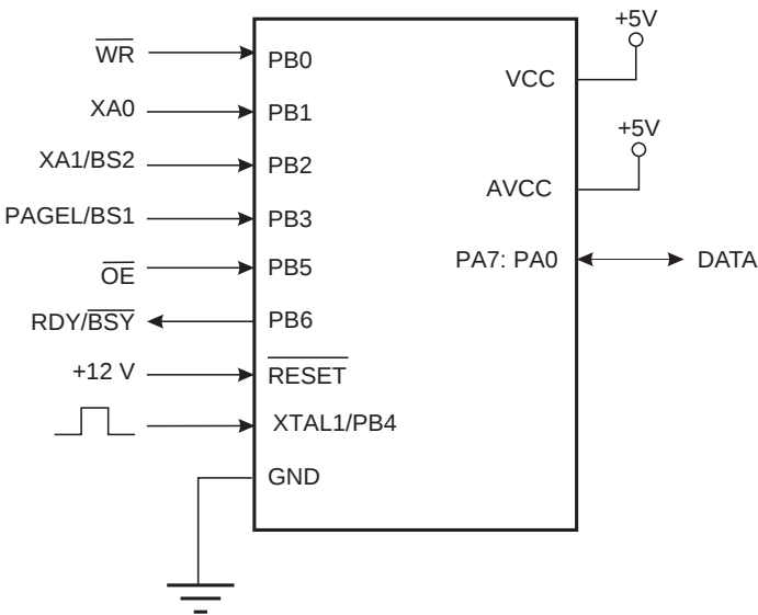
Figure 58. 并行编程
