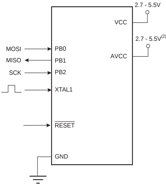
Figure 67. 串行编程及校验 (1)
