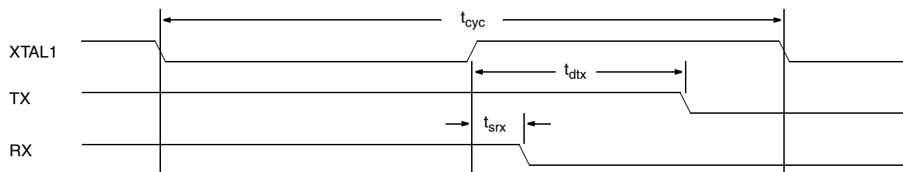
Fig. 3-3: CAN I/O Timing.
