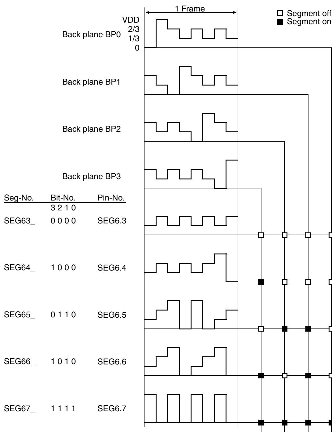
Fig. 17-3: Frame Timing Diagram
