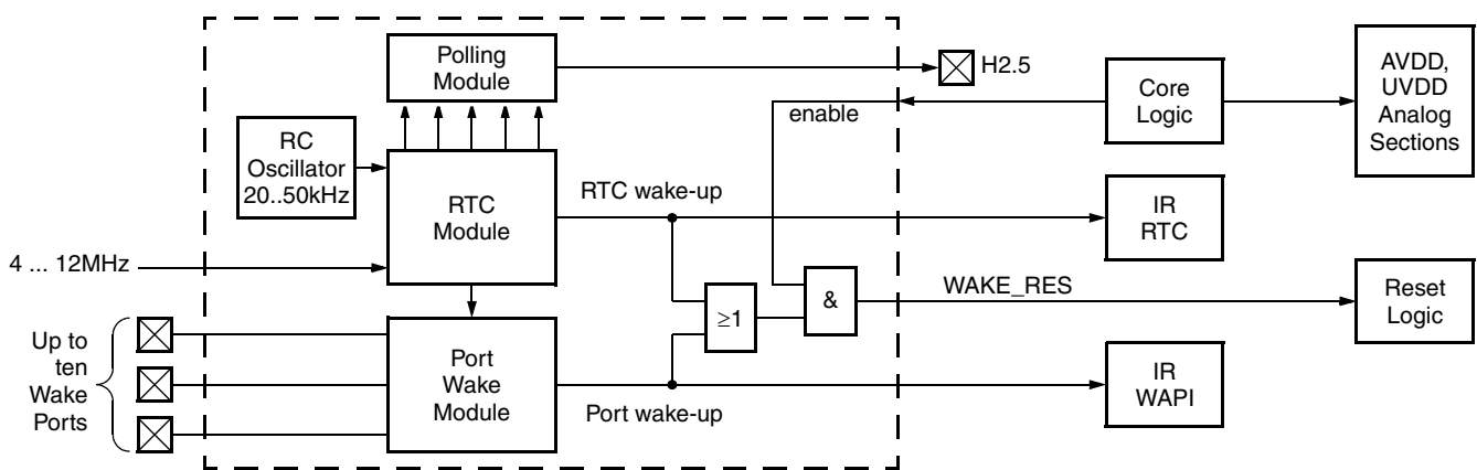
Fig. 8–1: Power-Saving Module
