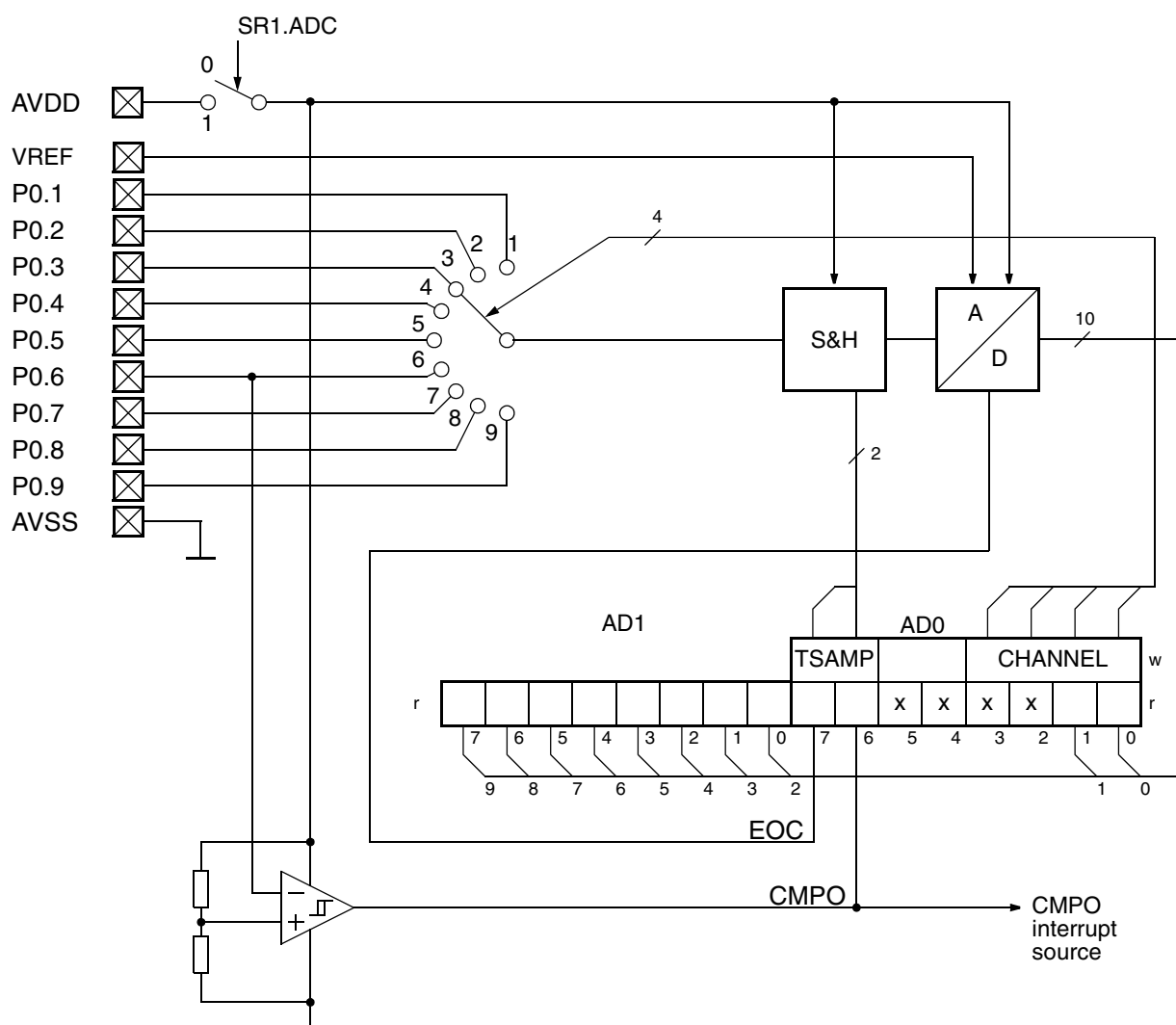
Fig. 12–1: Block Diagram
