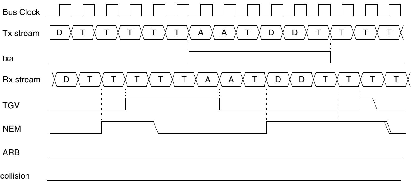
Fig. 23-7: Tx Timing
