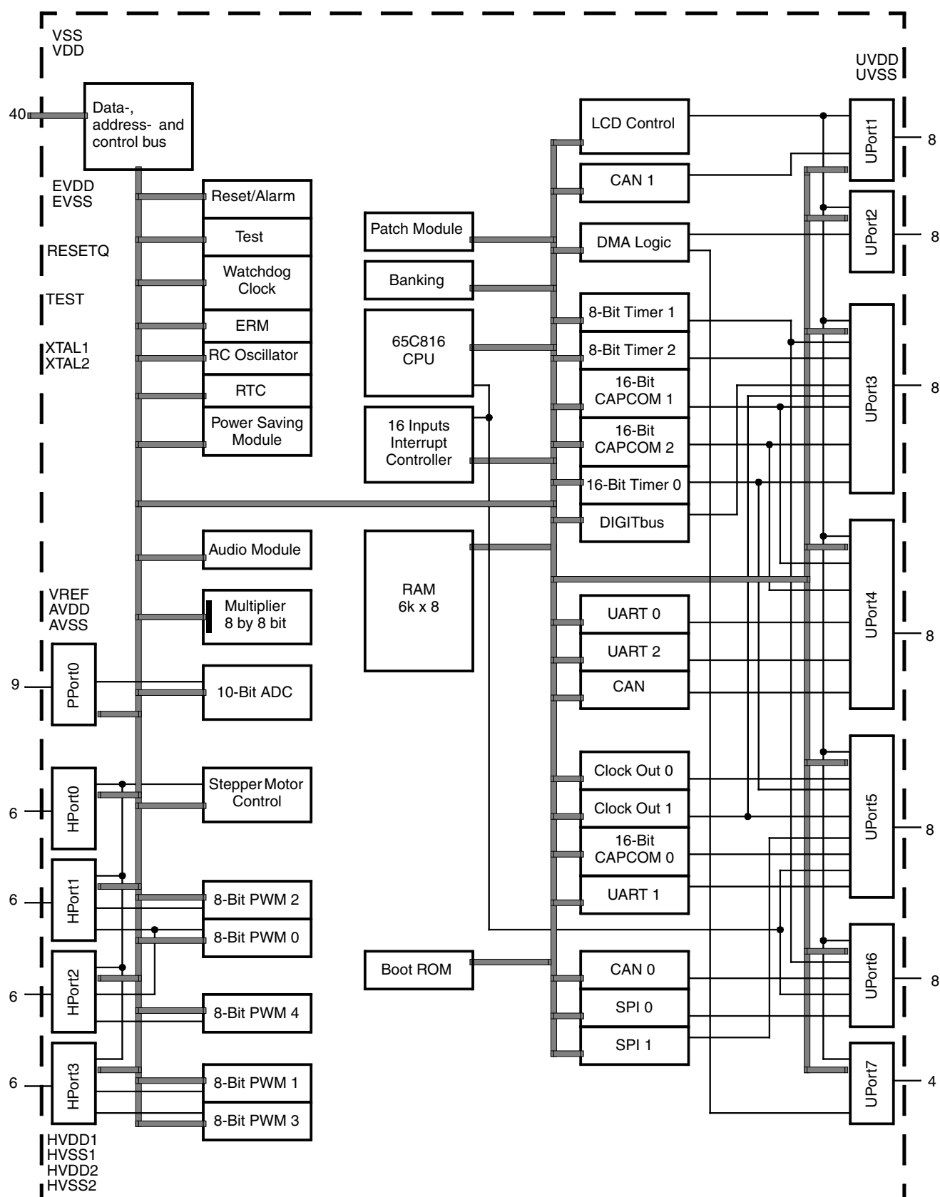
Fig. 1-1: Block diagram of CDC1605F-E
