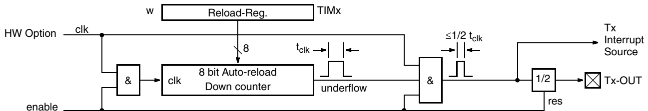
Fig. 13–3: Timer T1 and T2 Block Diagram
