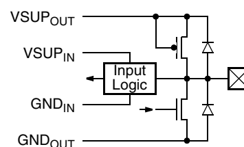
Fig. 2-8: Open Drain I/O
