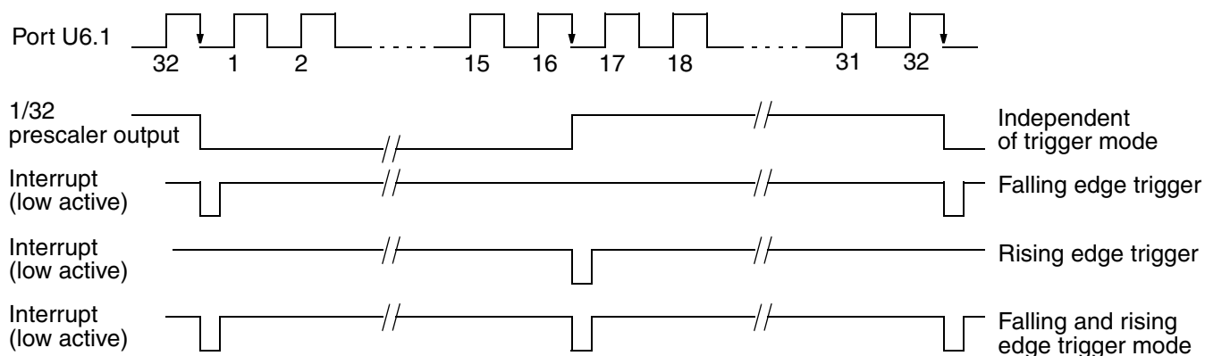
Fig. 10–7: Interrupt Timing (1/32 Prescaler On)
