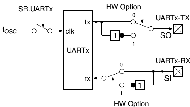
Fig. 20–2: Context Diagram
