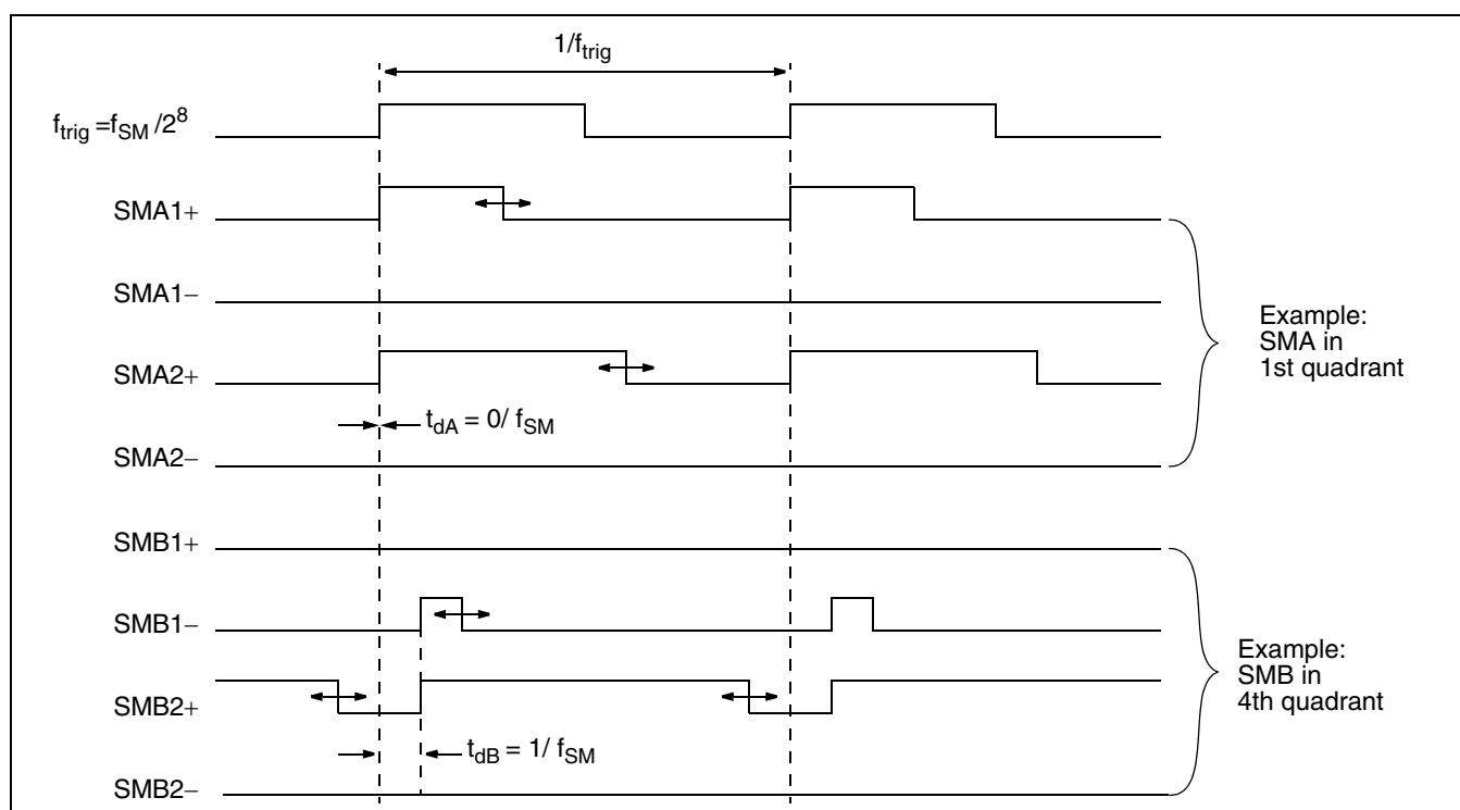
Fig. 16–1: Timing Diagram of Output Signals
