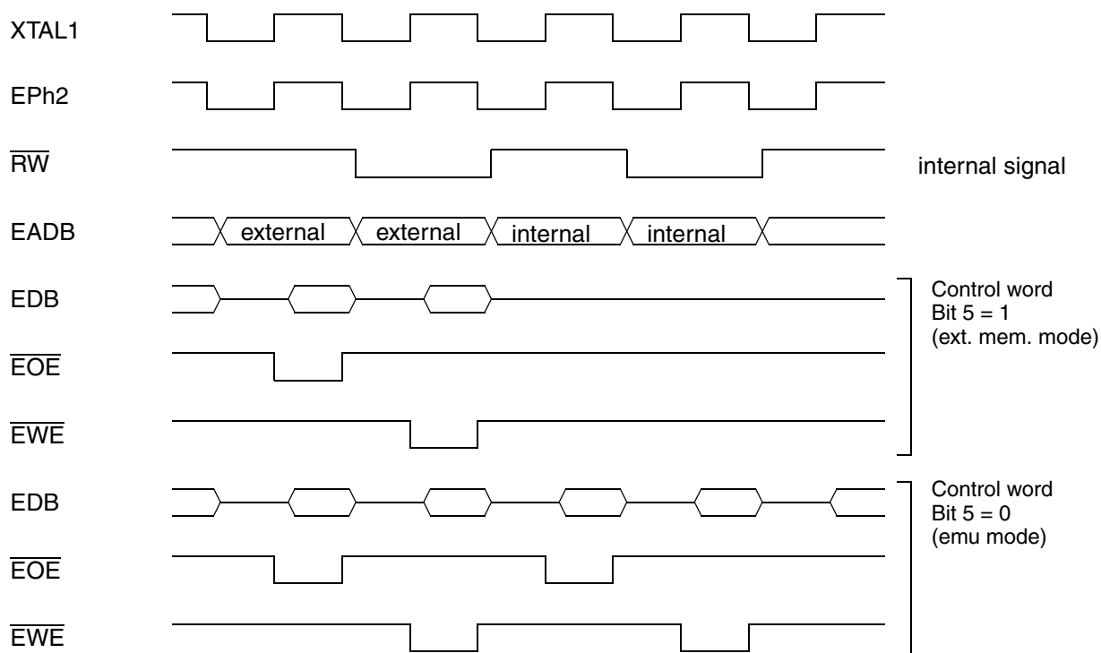
Fig. 3–8: Internal/External Memory Access
