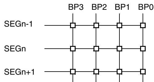
Fig. 17–1: Segments and Backplanes
