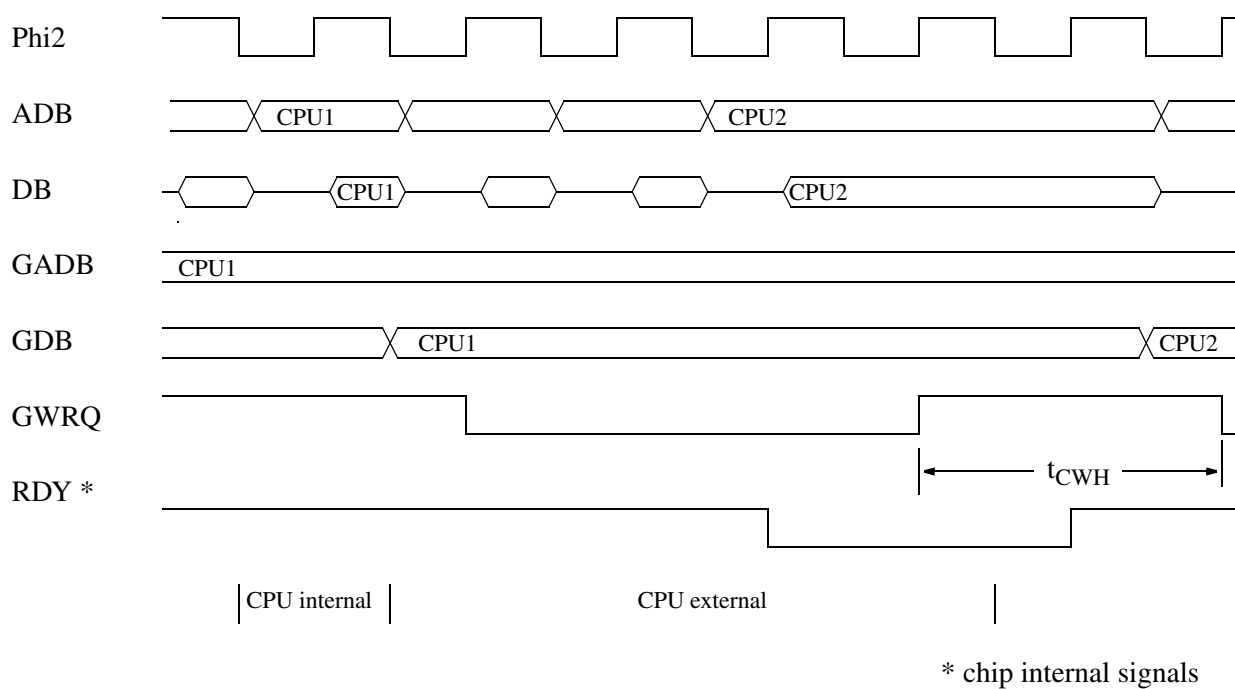
Fig. 18–6: CPU Write, WS = 4, with RDY because CPU rewrites to fast.
