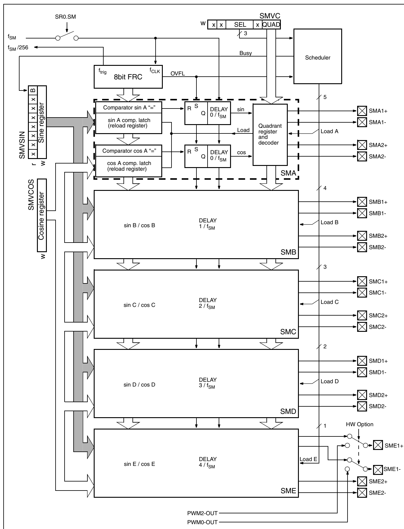
Fig. 16-2: Block Diagram of Output Generation Circuit
