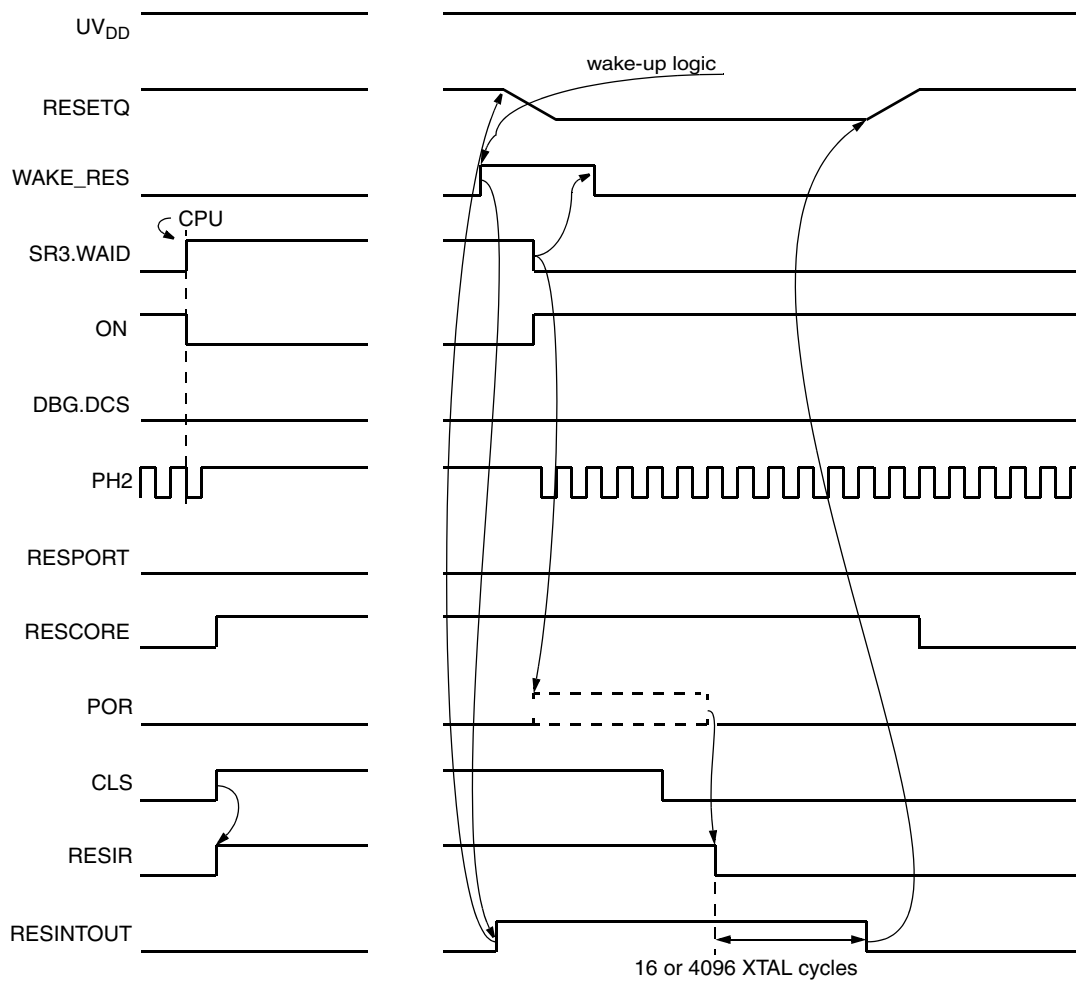
Fig. 8-4: Switching to WAKE/IDLE with DBG.DCS inactive and Wake-up
