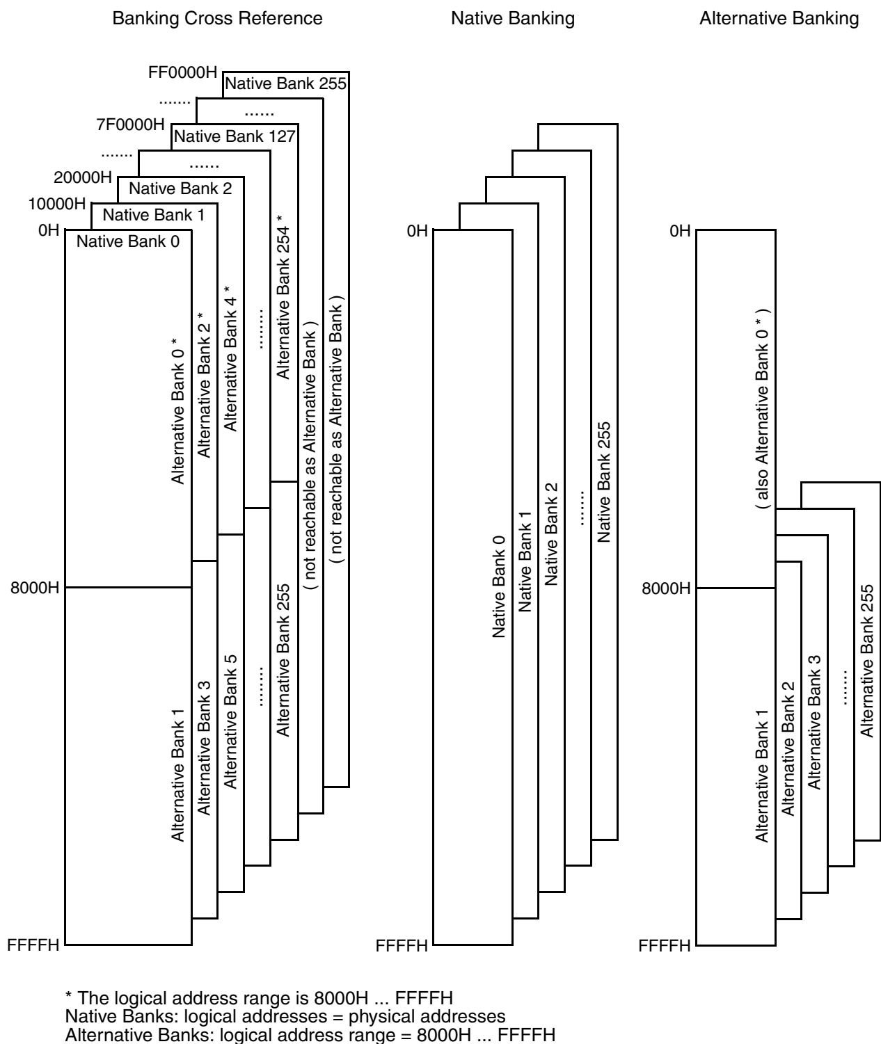
Fig. 5-4: Banking Map shown with the max. size of addressable memory (different from the implemented amount)
