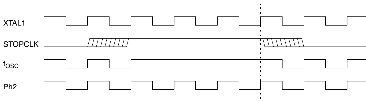
Fig. 3–7: Stop Clock (only if TEST Pin = 1)
