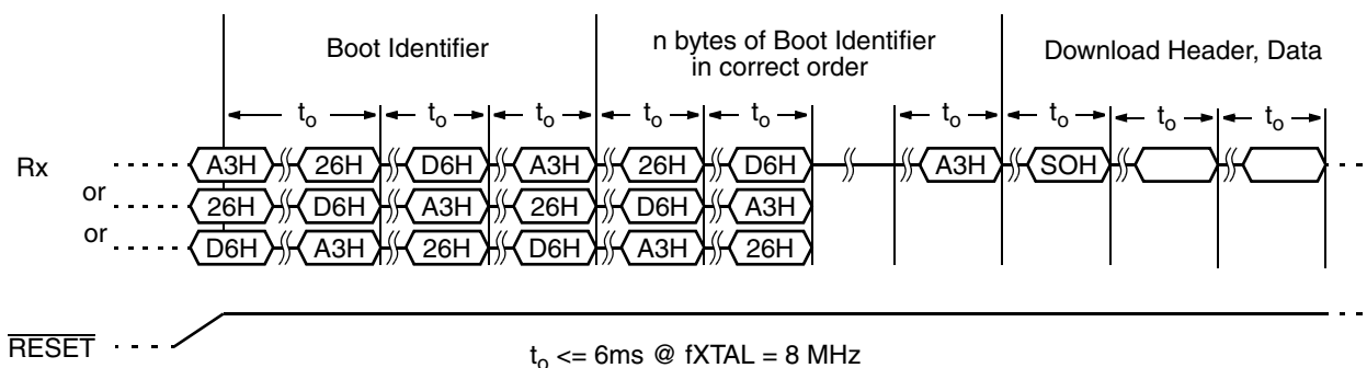
Fig. 5–8: UART Timing
