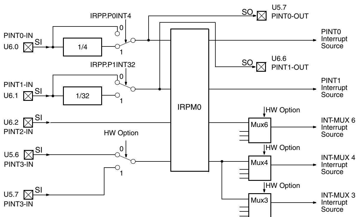
Fig. 10–5: Port Interrupts
