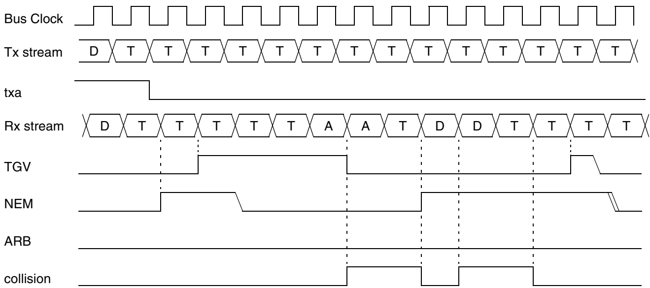
Fig. 23-8: Rx Timing
