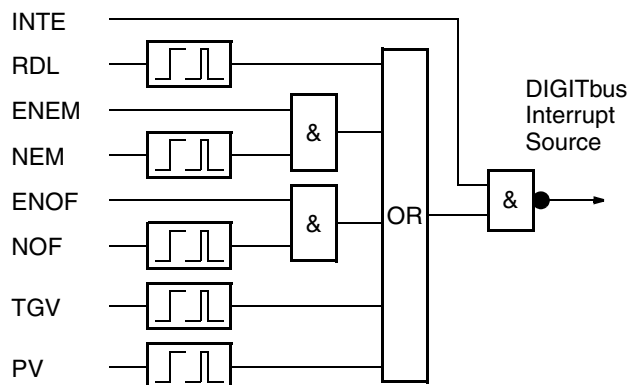
Fig. 23–6: Interrupt Sources
