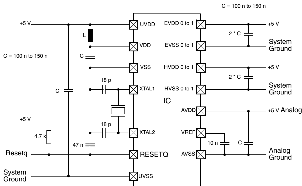
Fig. 2–4: Recommended external supply and quartz connection for low electromagnetic interference (EMI)
