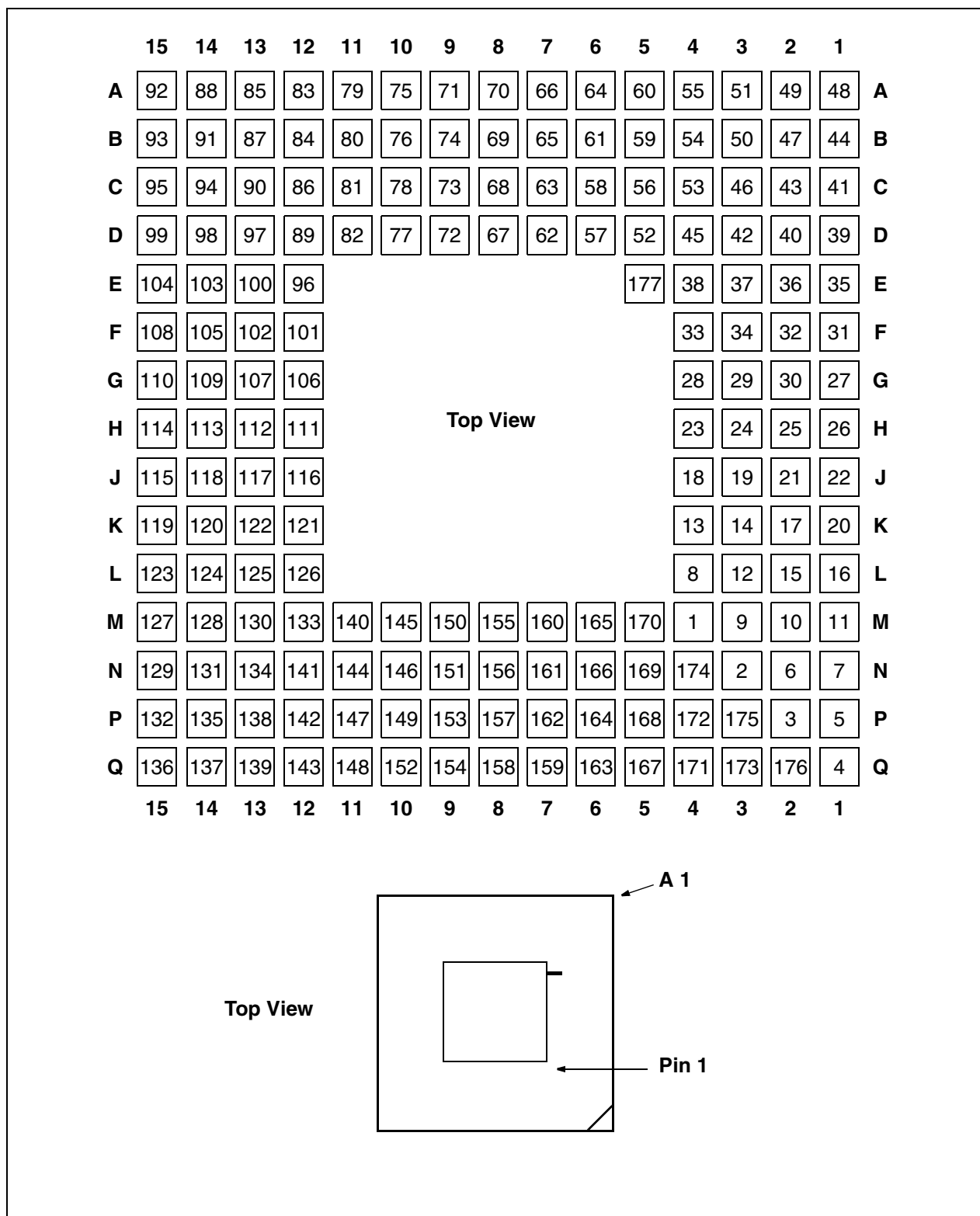
Fig. 2–1: Pin Map of CPGA177 Package
