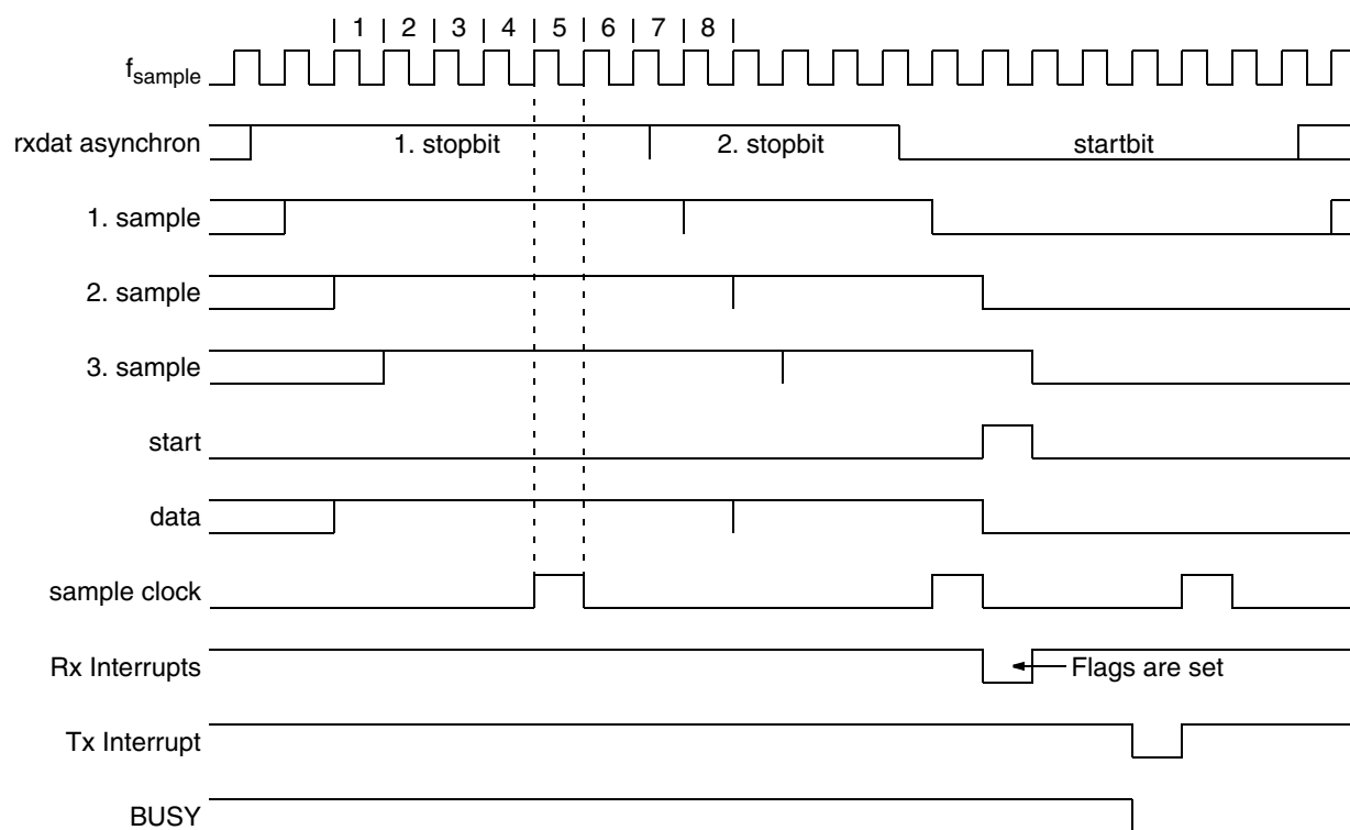
Fig. 20-5: End of Telegram
