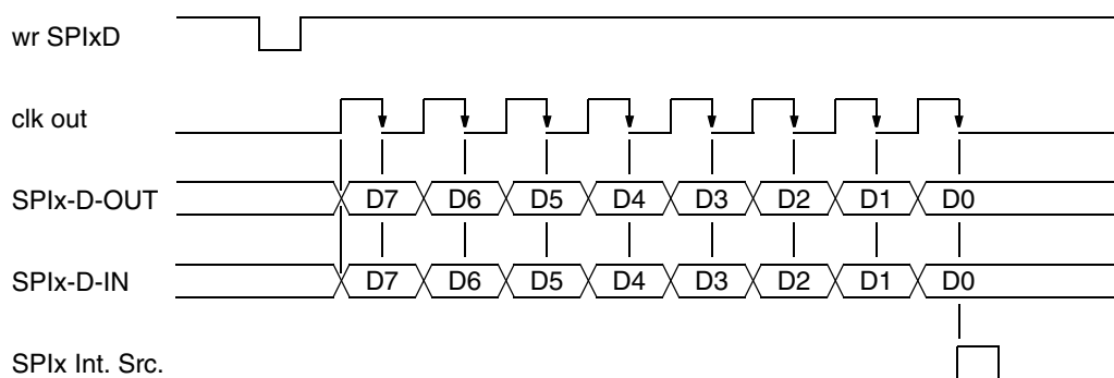
Fig. 19–3: Eight bit frame. Data valid at falling edge.
