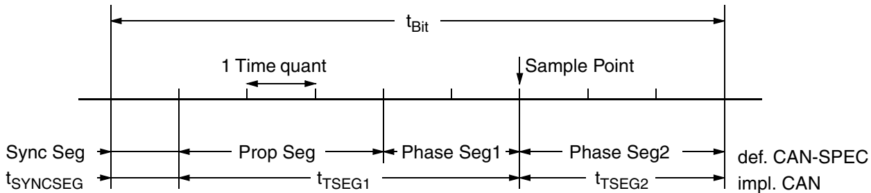
Fig. 21–10: Bit Timing Definition
