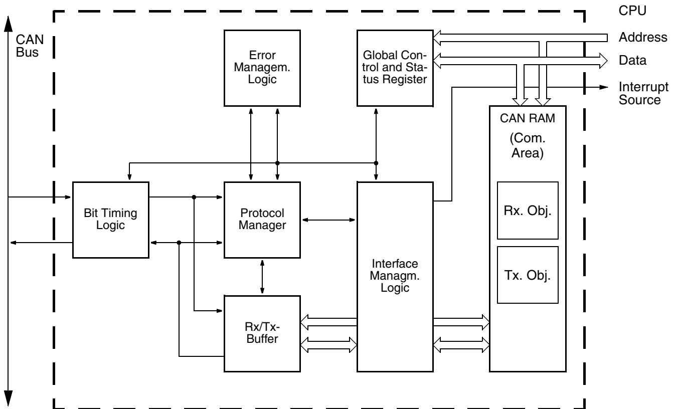
Fig. 21-1: Block diagram of the CAN bus interface
