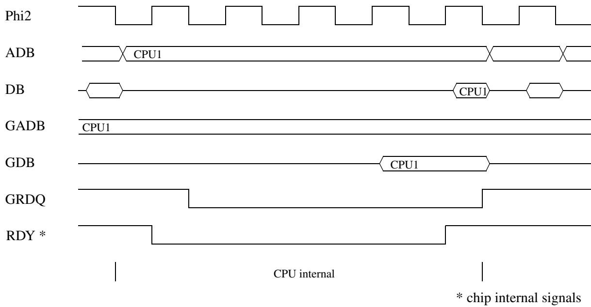
Fig. 18–8: CPU Read, WS = 4
