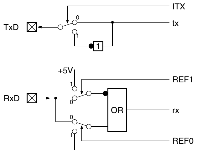
Fig. 21–11: Bus Coupling
