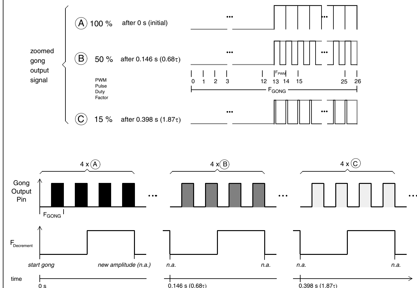
Fig. 24–2: Example sections of the audio module output signal
