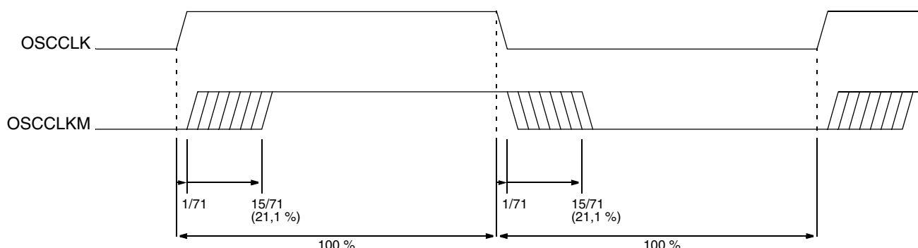
Fig. 4–5: Timing of modulated clock
