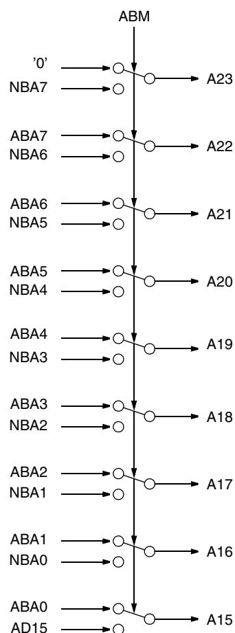
Fig. 5-3: Physical Address change depending on the Banking Mode
