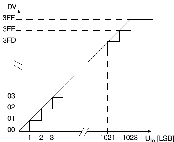
Fig. 12-2: Characteristic Curve
