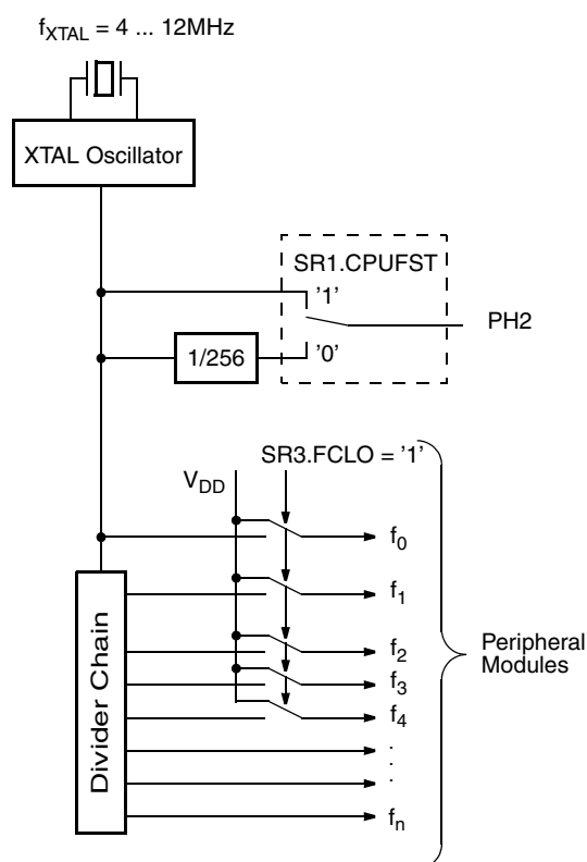
Fig. 4–2: Clock System
