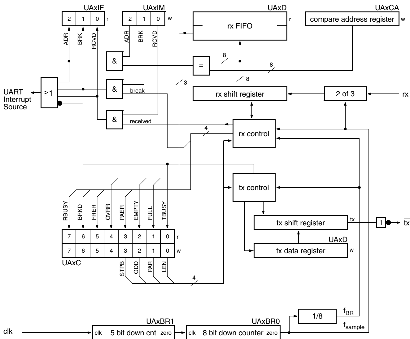
Fig. 20–1: Block Diagram
