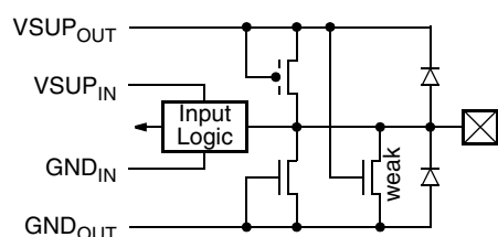
Fig. 2-6: Input Pins with Pull-Down
