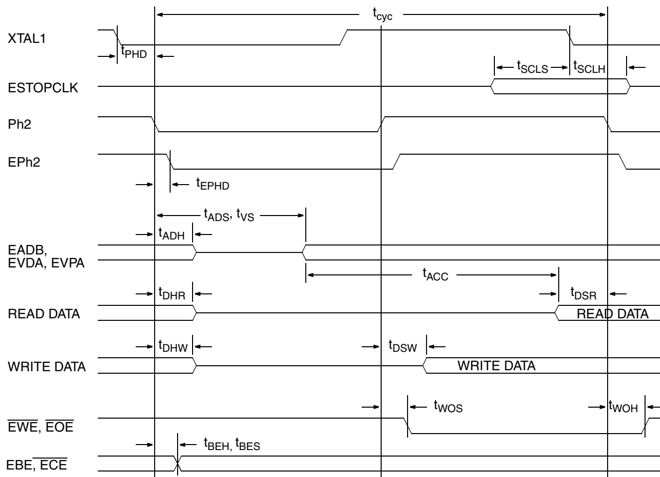
Fig. 3-5: Emu Bus Timing
