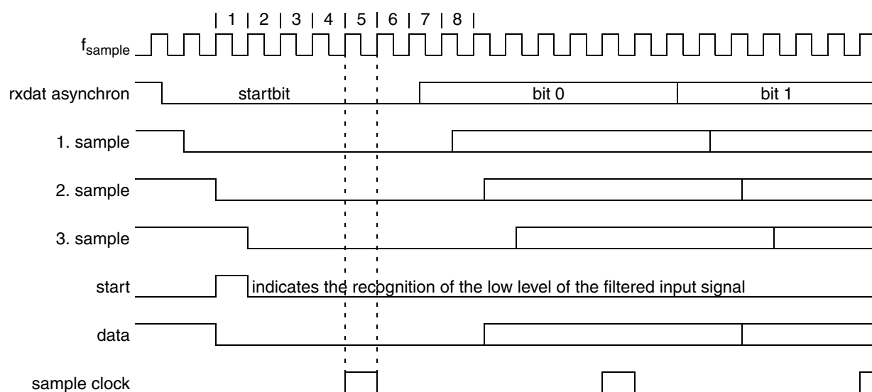
Fig. 20-4: Start of Telegram
