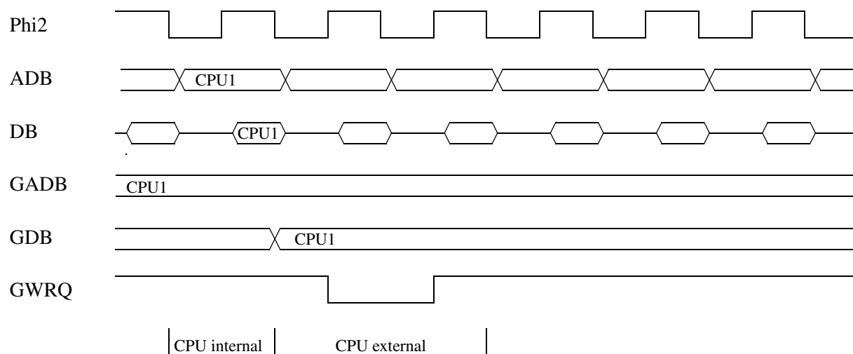
Fig. 18-5: CPU Write, WS = 2
