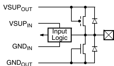
Fig. 2-5: Input Pins
