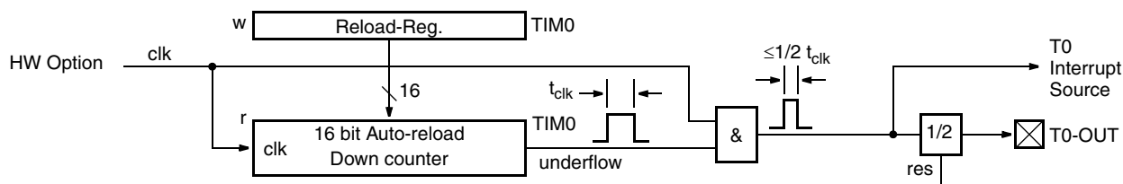
Fig. 13–1: Timer T0 Block Diagram
