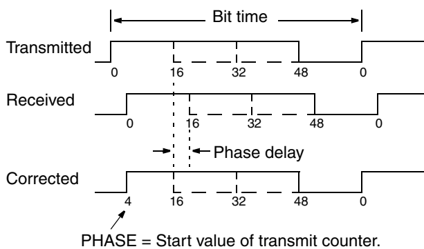
Fig. 23–3: Phase Correction
