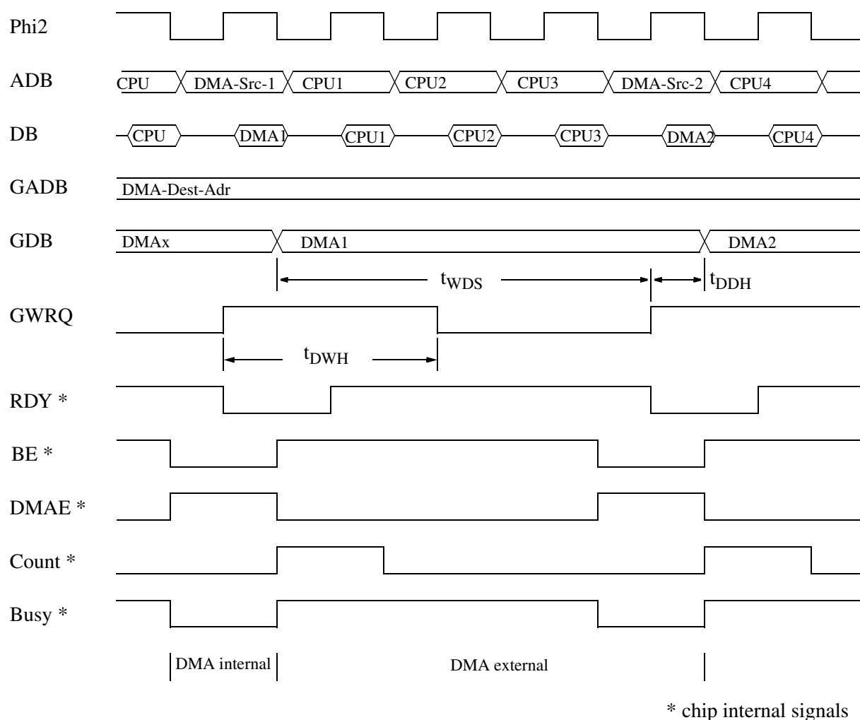
Fig. 18-4: DMA Write, WS = 4
