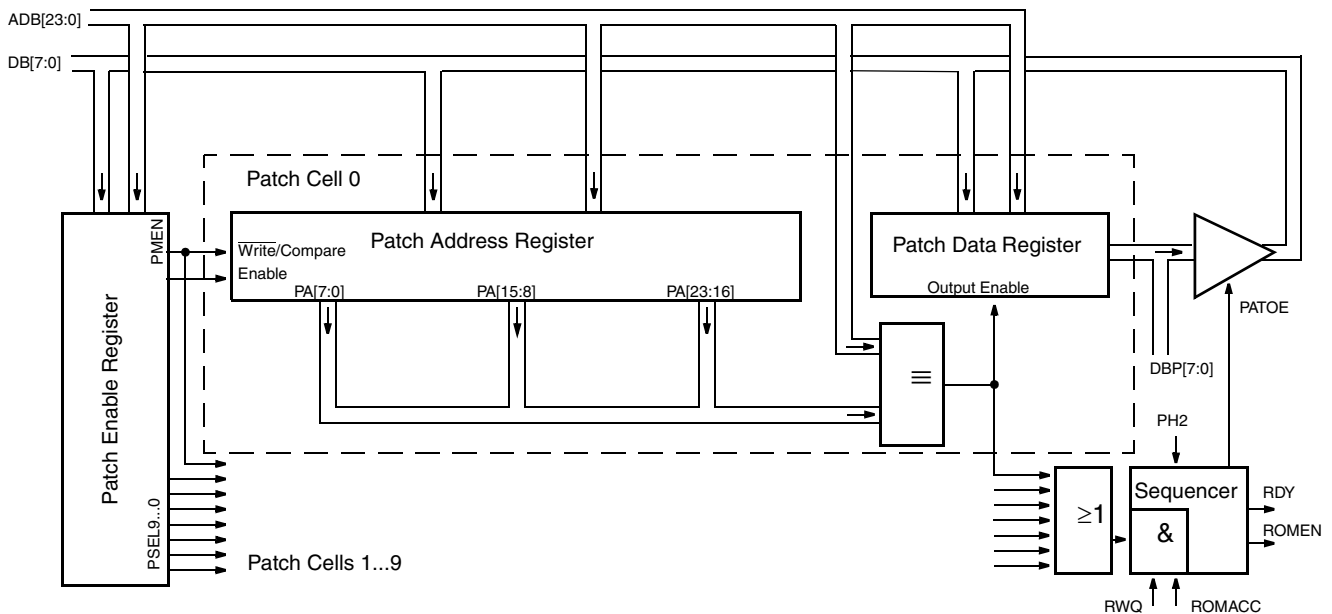
Fig. 9-1: Block Diagram
