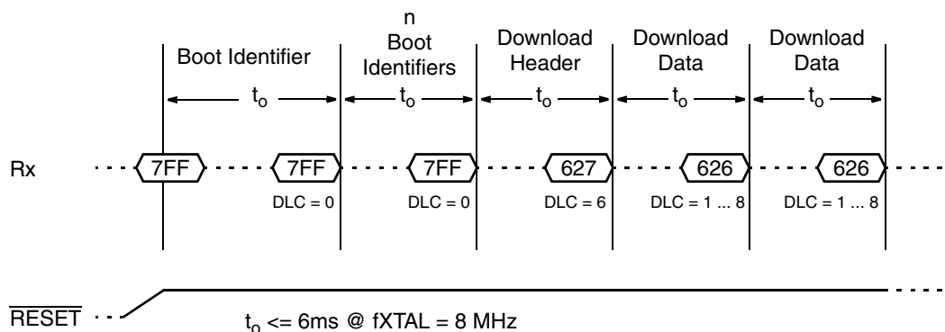
Fig. 5–9: CAN Timing
