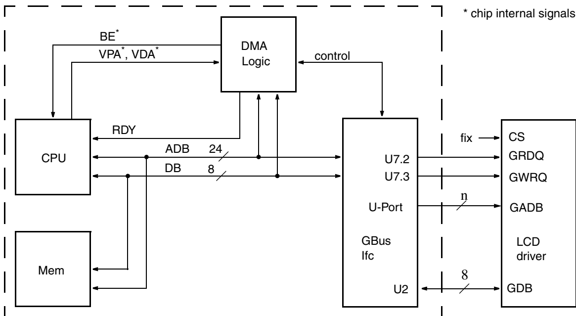
Fig. 18–1: Block Diagram
