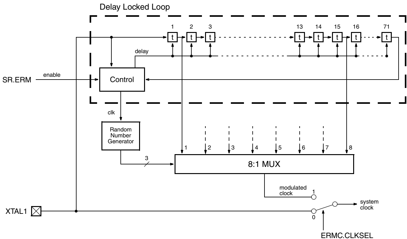
Fig. 4–4: Block Diagram
