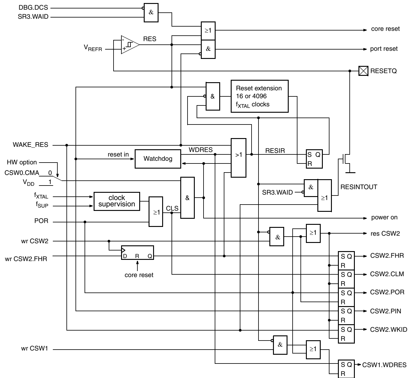
Fig. 6-2: Reset Logic Block Diagram
