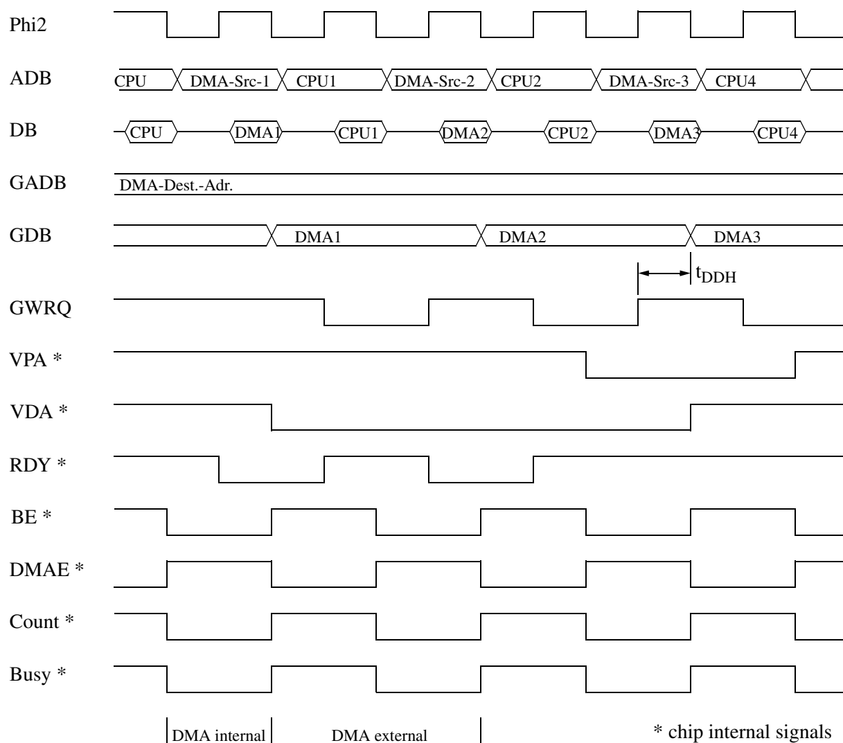
Fig. 18–3: DMA Write, WS = 2
