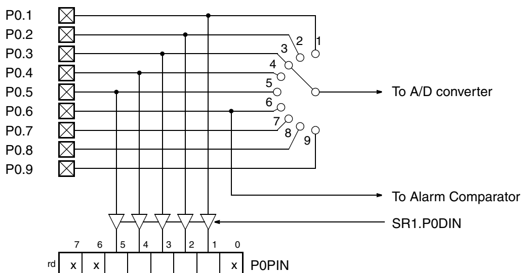
Fig. 11–1: Port 0 with Input Multiplexer and Undervoltage Alarm Comparator
