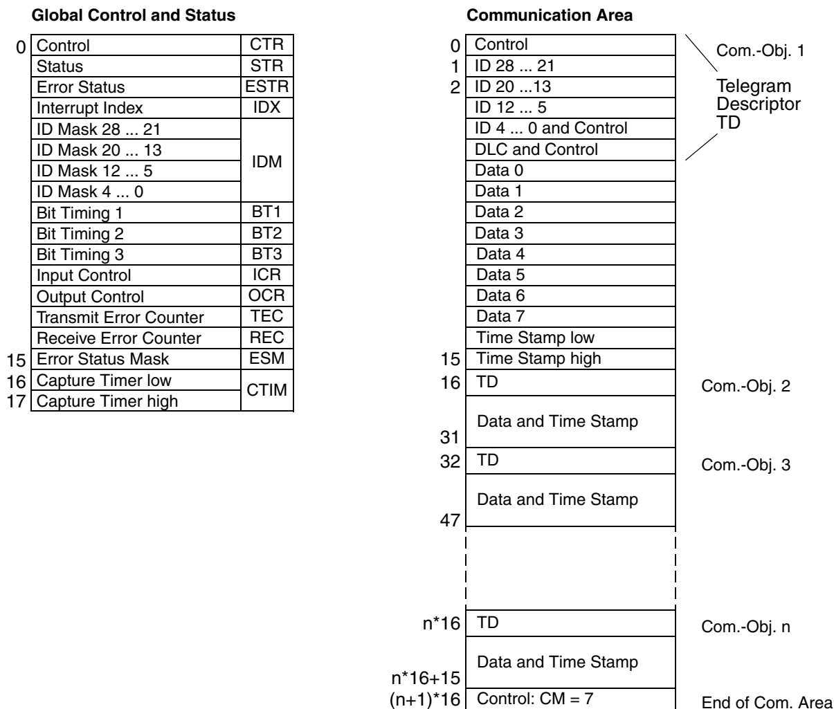
Fig. 21-2: Memory allocation
