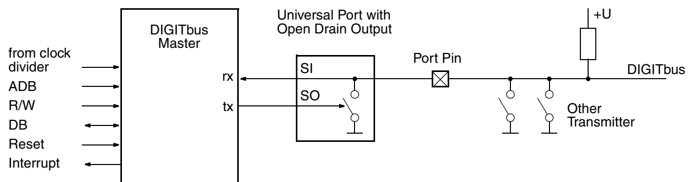
Fig. 23–1: Context Diagram
