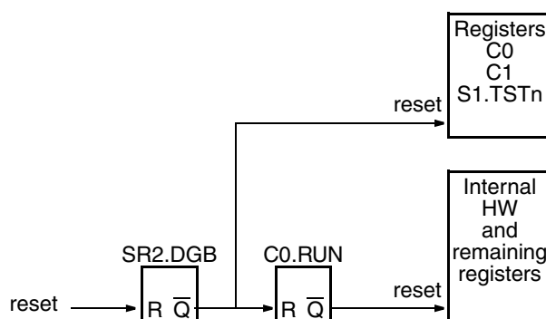
Fig. 23–5: Reset Structure
