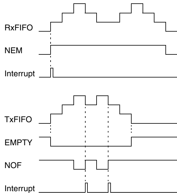
Fig. 23–4: Rx- and TxFIFO Timing
