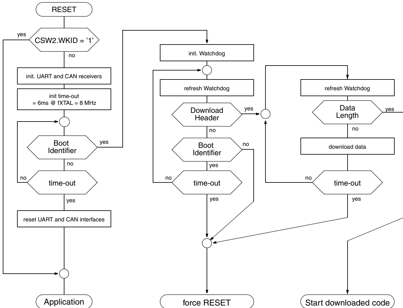
Fig. 5-7: Boot Loader flow-chart
