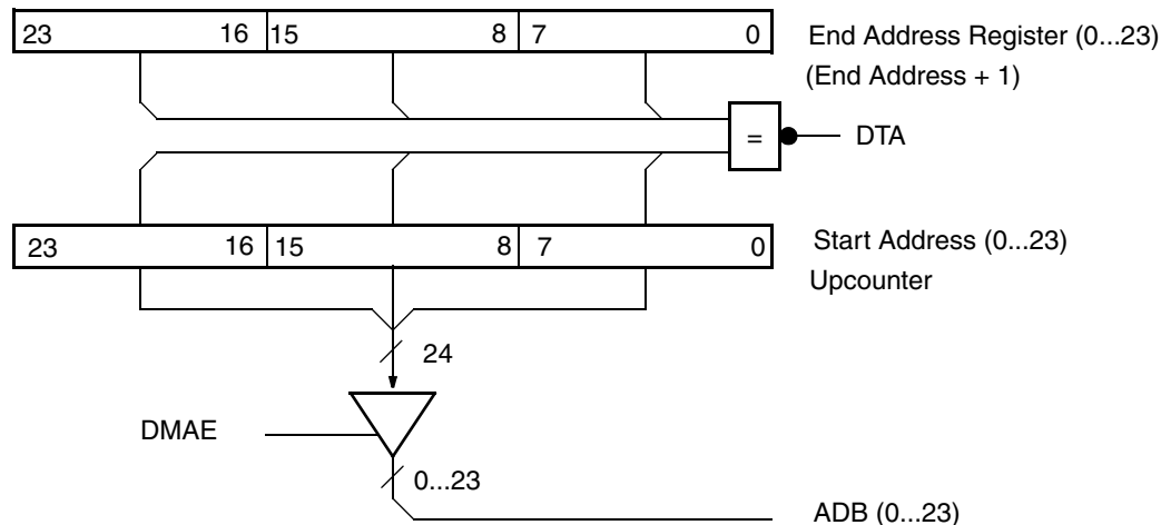
Fig. 18–2: DMA Address Generator
