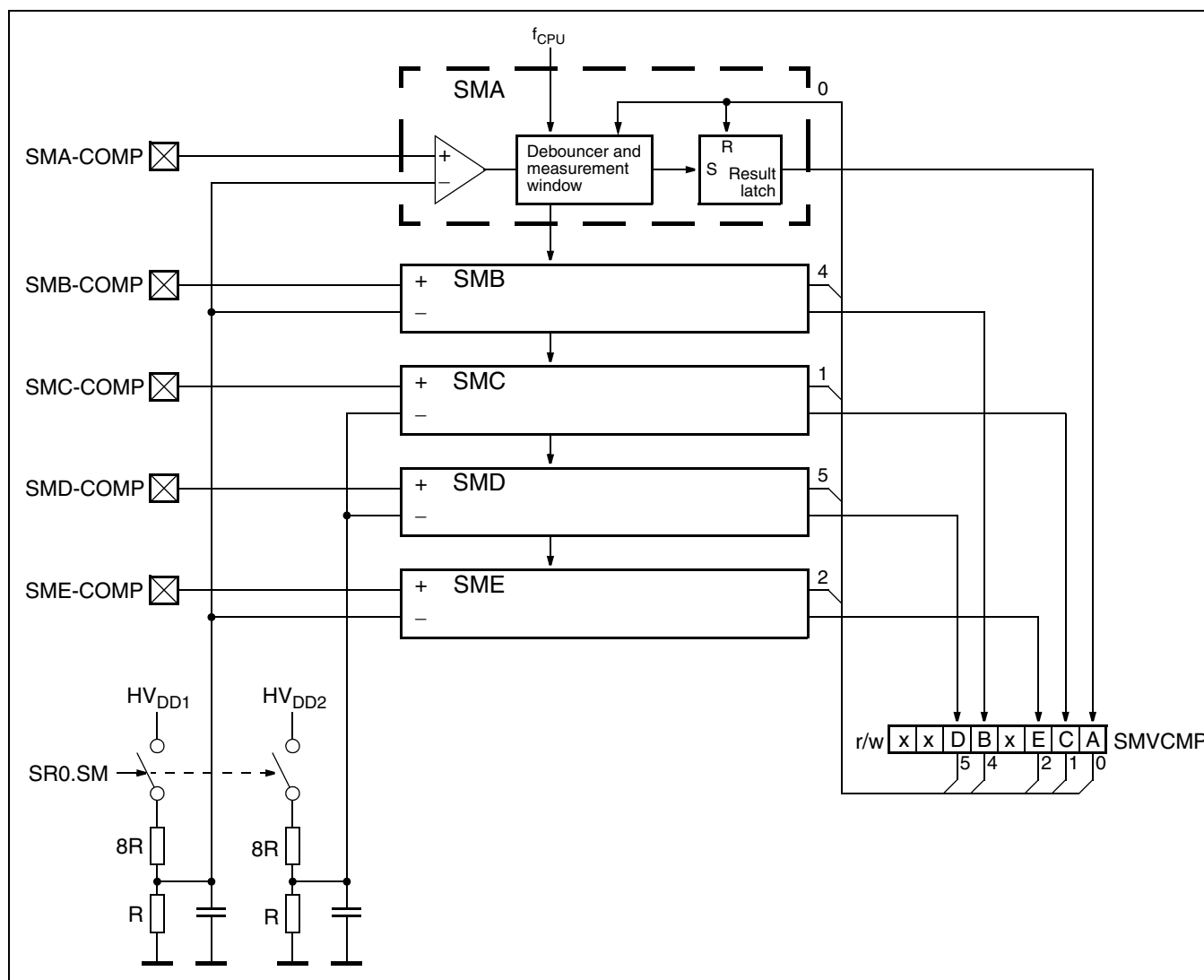
Fig. 16-3: Block Diagram of Rotor Zero Position Detection Circuit
