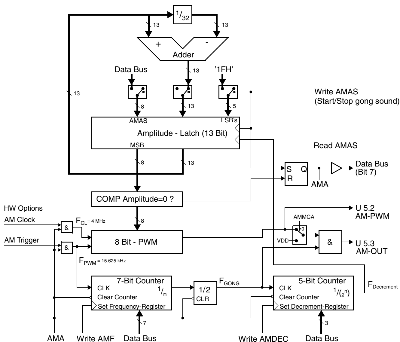
Fig. 24–1: Block diagram of the audio module
