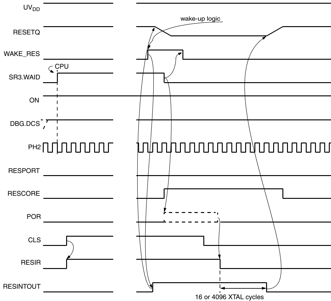
Fig. 8-5: Switching to WAKE/IDLE with DBG.DCS active and Wake-up
