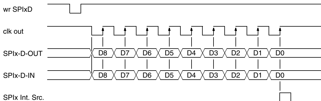
Fig. 19–2: Nine bit frame. Data valid at rising edge.
