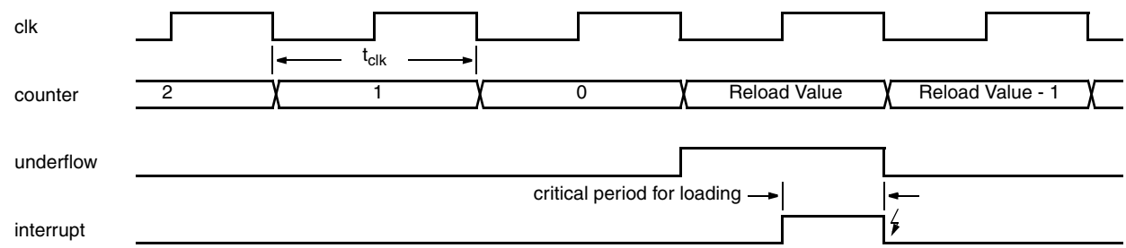
Fig. 13–2: Timer0 Timing
