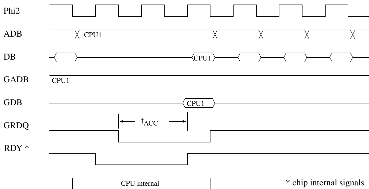
Fig. 18–7: CPU Read, WS = 2
