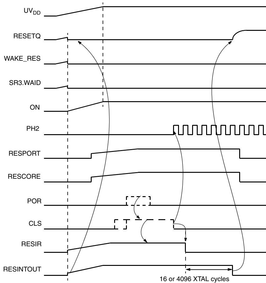
Fig. 8-3: Power-on Reset
