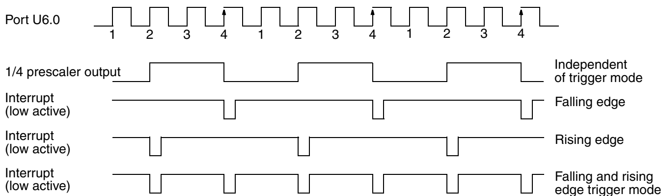
Fig. 10–6: Interrupt Timing (1/4 Prescaler On)
