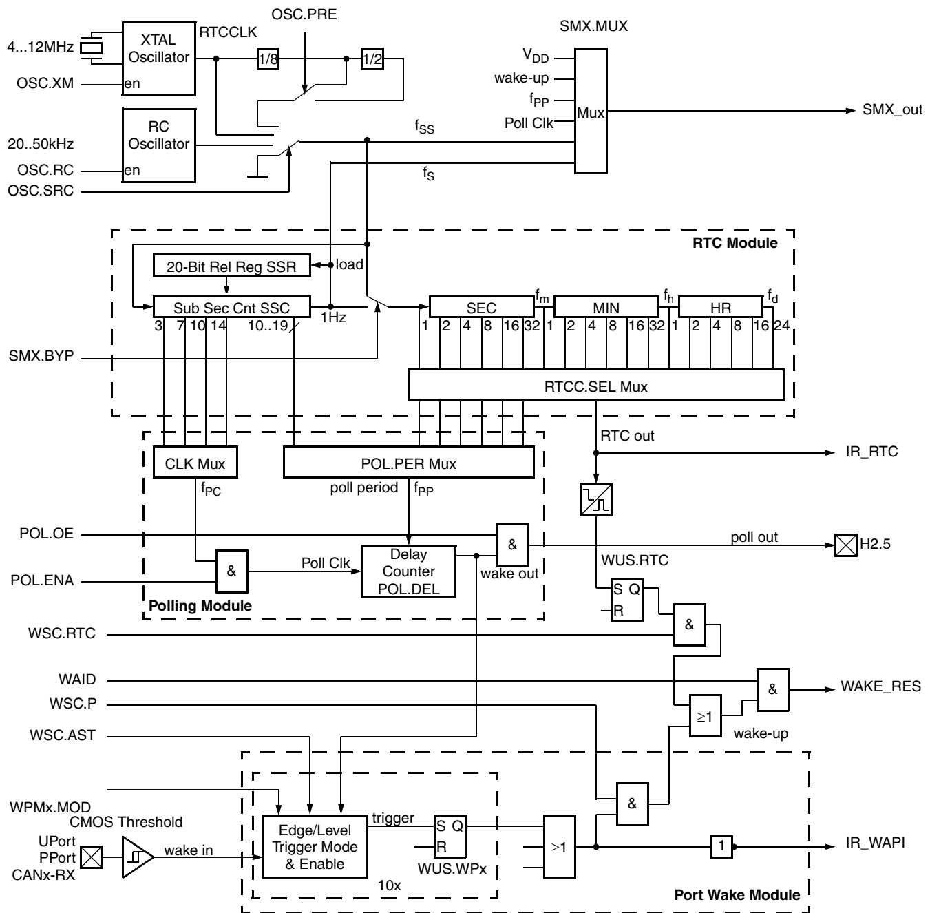
Fig. 8-2: Power-Saving Module Block Diagram
