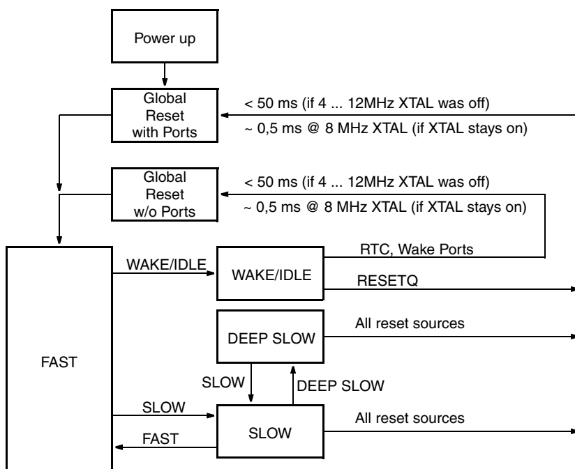
Fig. 4–1: Operating Modes State Diagram
