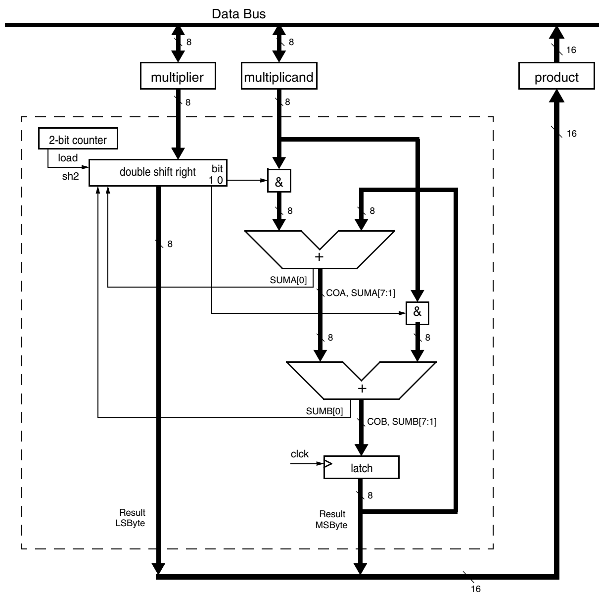
Fig. 7-1: Block diagram of the multiplier
