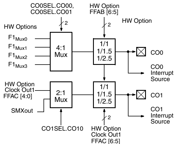
Fig. 4–3: Clock Outputs Diagram
