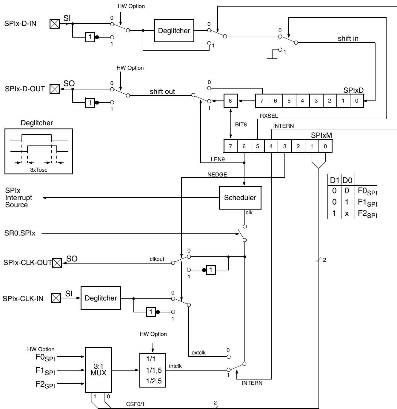
Fig. 19–1: Block Diagram
