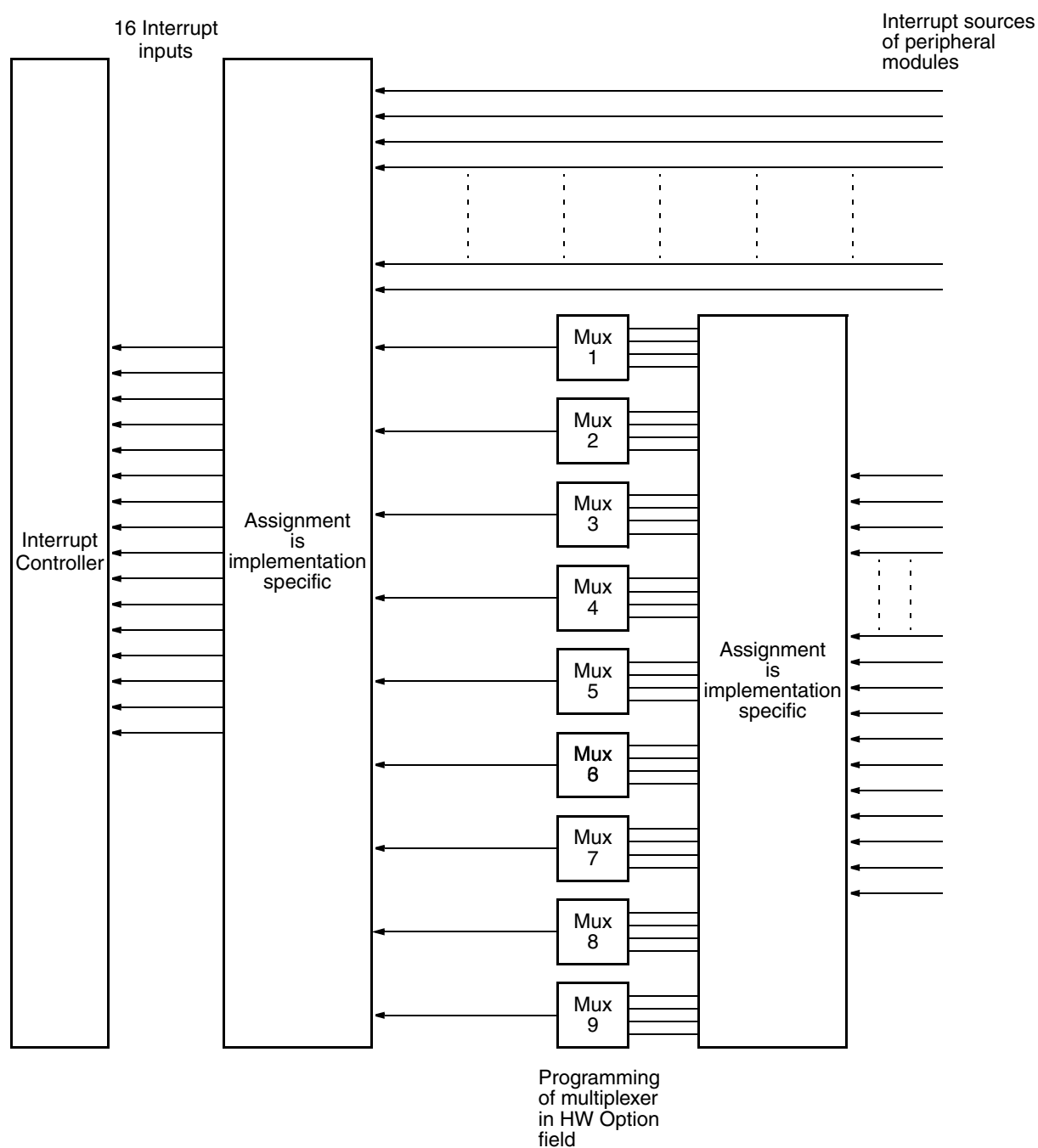
Fig. 10–3: Interrupt Assignment and Multiplexer
