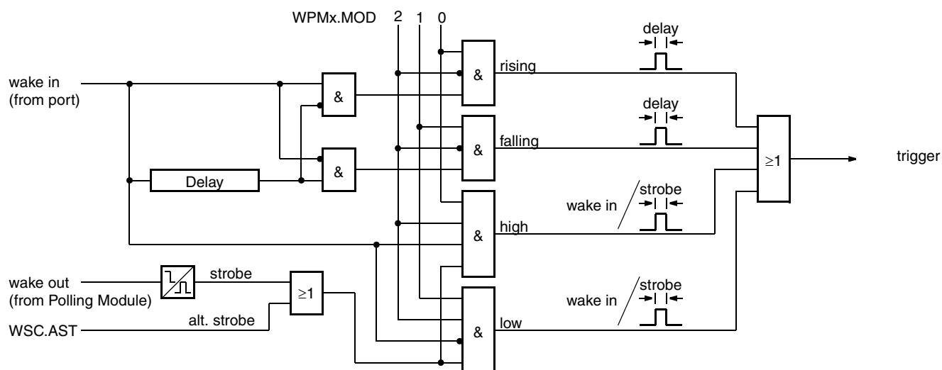
Fig. 8–7: Edge/Level Trigger Logic
