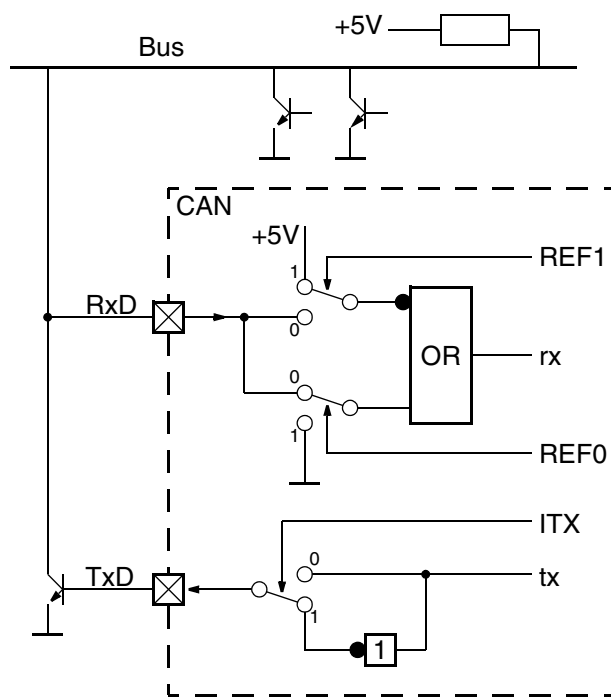
Fig. 21–12: Minimum Bus
