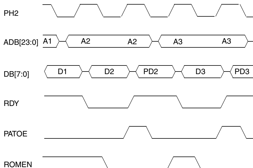
Fig. 9–2: Timing
