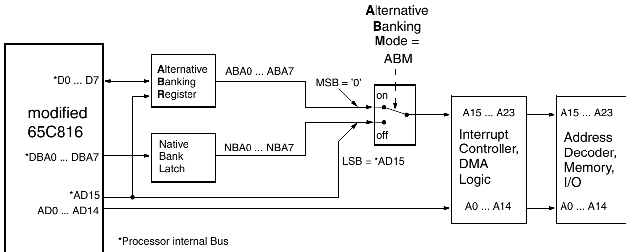
Fig. 5-2: Block diagram Memory Banking
