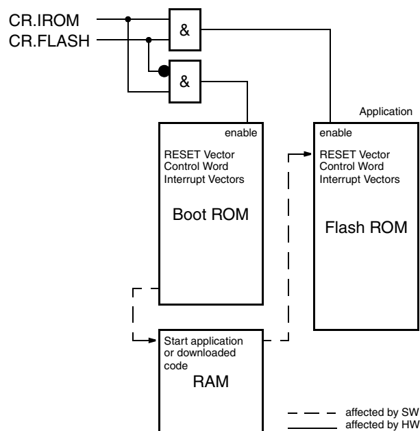
Fig. 5–6: Boot ROM Selection
