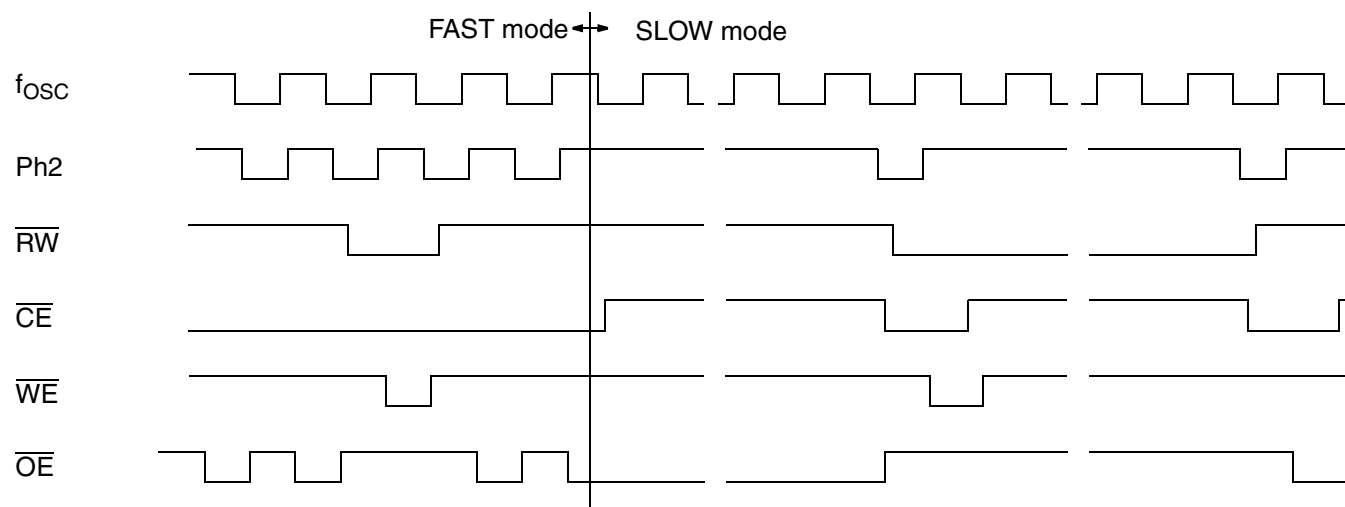
Fig. 3-6: Memory Access Signals
