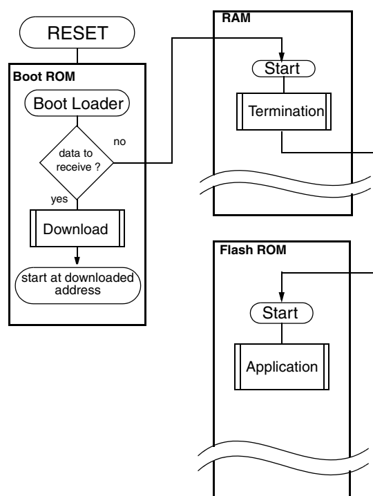
Fig. 5–5: Principle of the boot system
