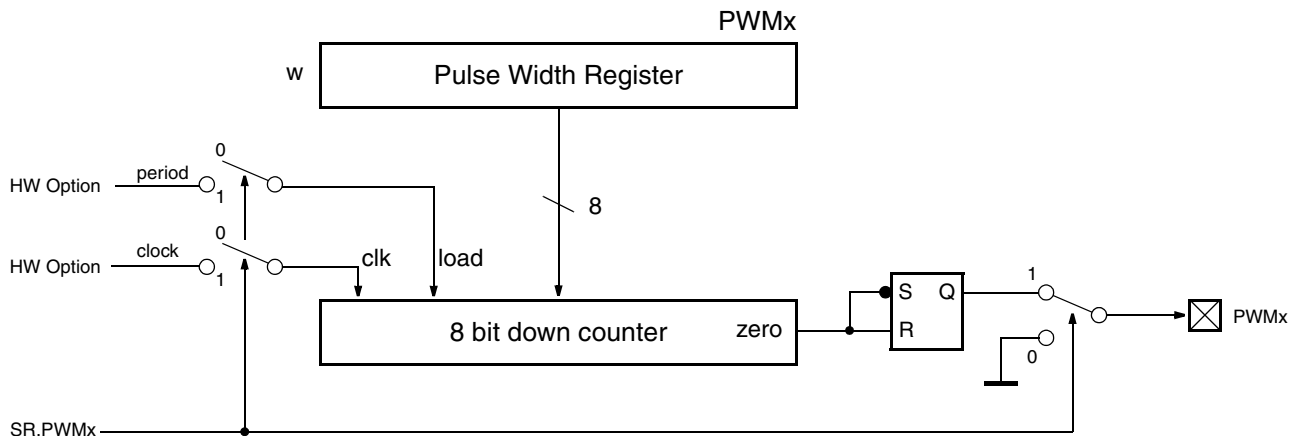
Fig. 14–1: PWM Block Diagram
