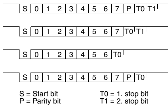
Fig. 20–3: Examples of Telegram Formats
