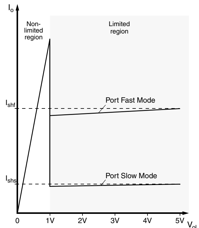
Fig. 11–3: Typical U-Port pull-down DC output characteristic (pull-up characteristic is complementary).
