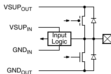
Fig. 2-7: Push Pull I/O Pins
