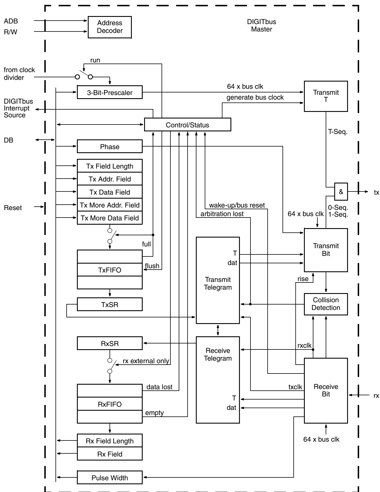
Fig. 23-2: Block Diagram
