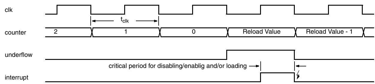
Fig. 13–4: Timer1 and 2 Timing
