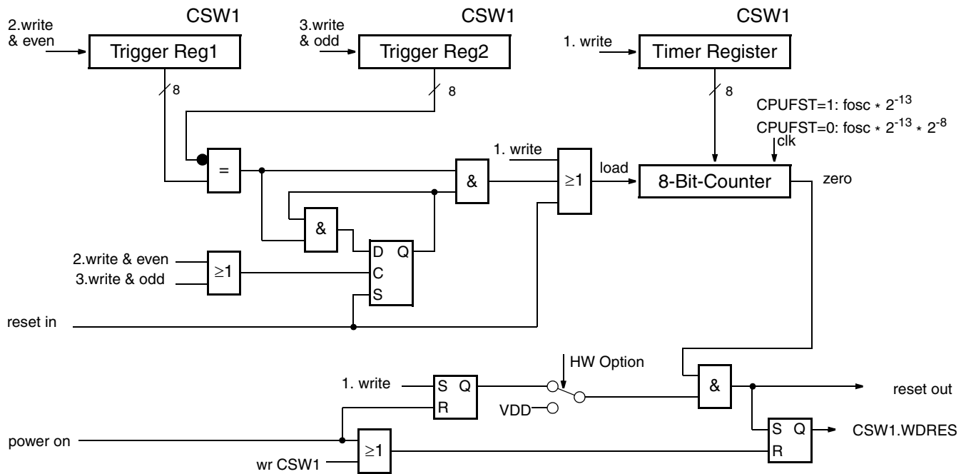
Fig. 6–3: Watchdog Block Diagram
