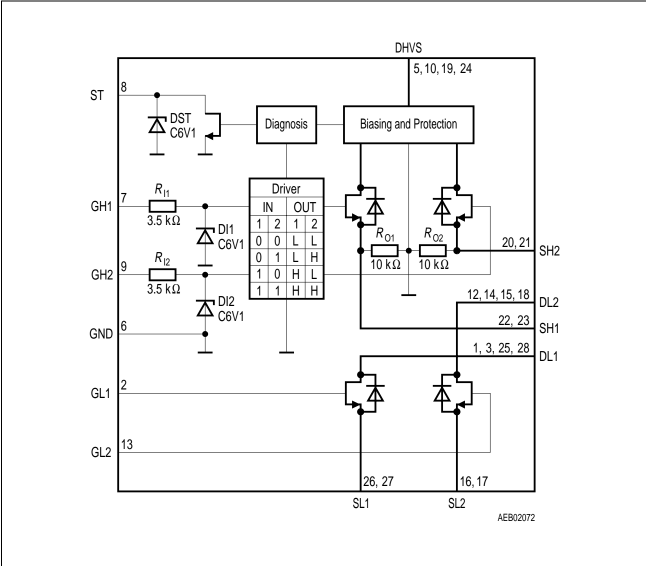
Figure 2 Block Diagram
