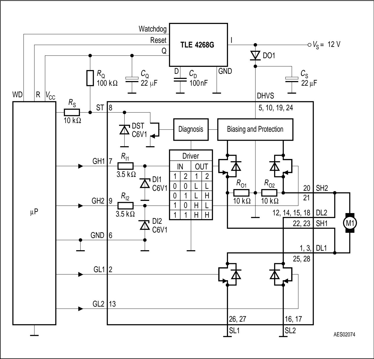
Figure 4 Application Circuit
