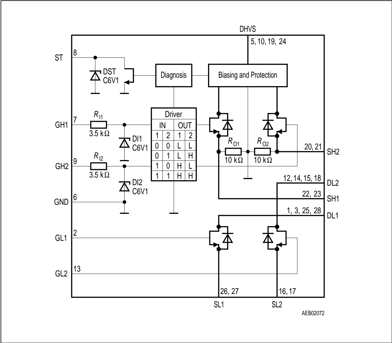
Figure 2 Block Diagram
