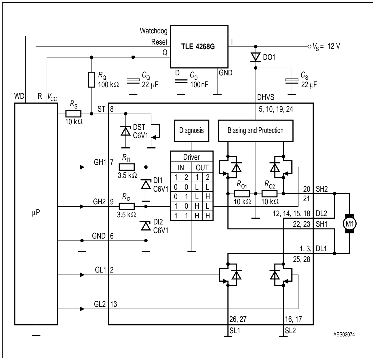
Figure 4 Application Circuit
