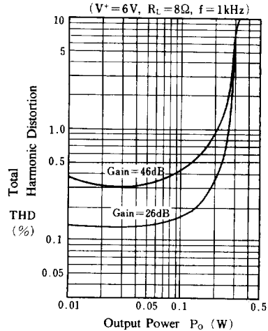
Total Harmonic Distortion vs. Output Power ( V^+ = 6\text{V} , R_L = 8\Omega , f = 1\text{kHz} )
