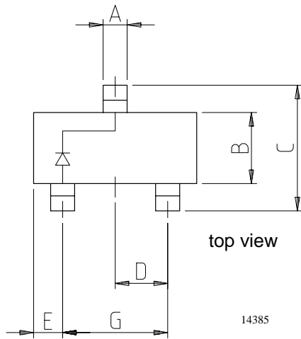
BAT54
