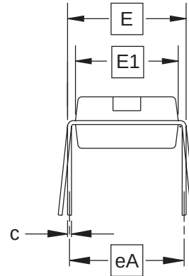
End View
