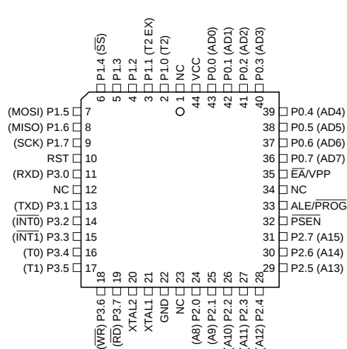
PLCC Top View
