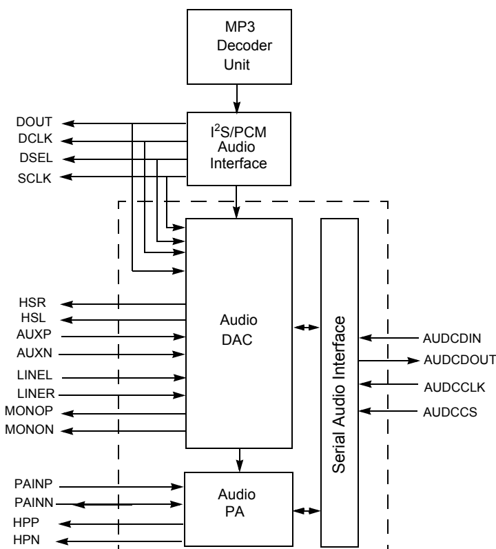
Figure 19. Audio Interface Block Diagram
