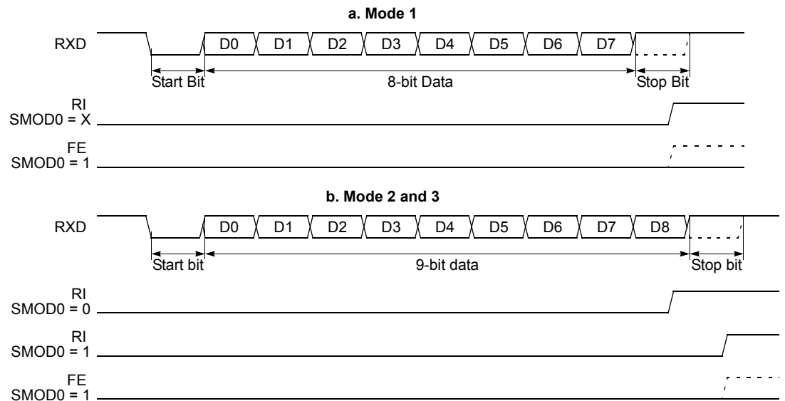
Figure 73. Interrupt Waveforms
