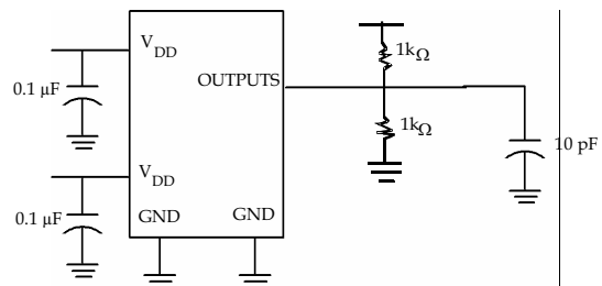
Test Circuit #2
