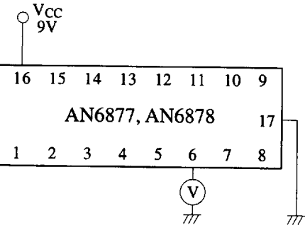
Test Circuit 3 (V REF )
