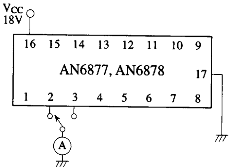
Test Circuit 6 (I Bias2 , I Bias3 )
