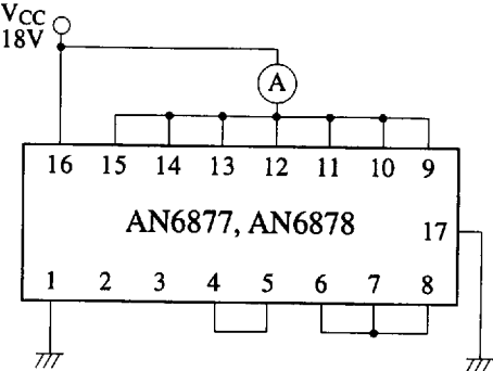
Test Circuit 5 (I 9-15 )
