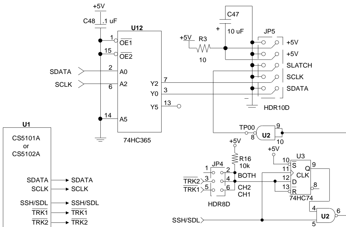
Figure 5. CDB5102A Evaluation Board Schematic for the Digital Interface
