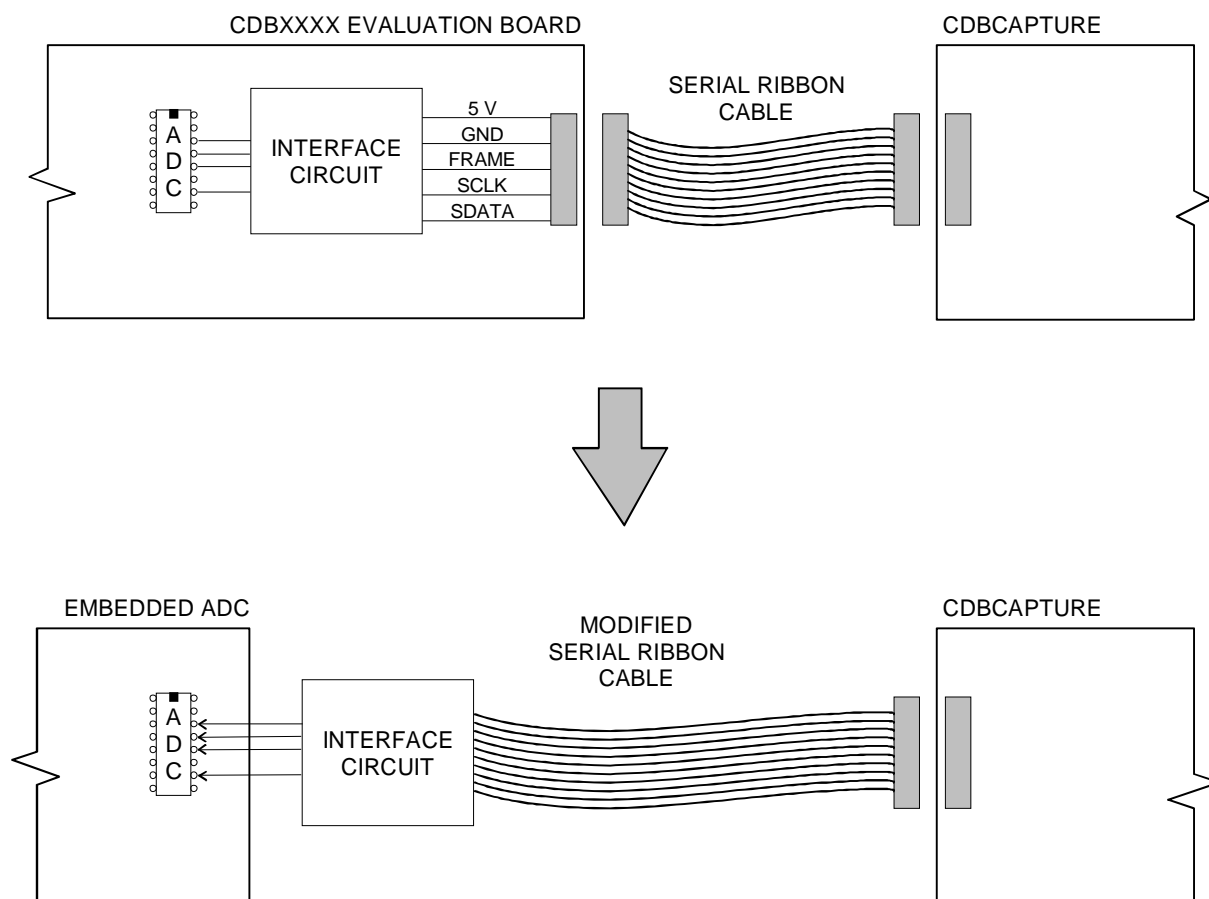
Figure 1. CDBCAPTURE INTERFACE
