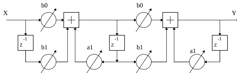
Figure 2. Filter Topology
