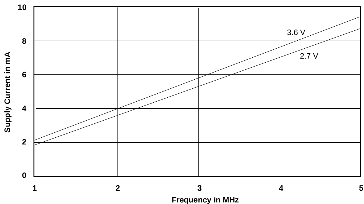
Figure 8. Typical I_{CC1} vs. Frequency
