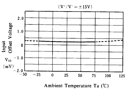
Input Offset Voltage vs. Temperature
