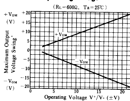
Maximum Output Voltage Swing vs. Operating Voltage
