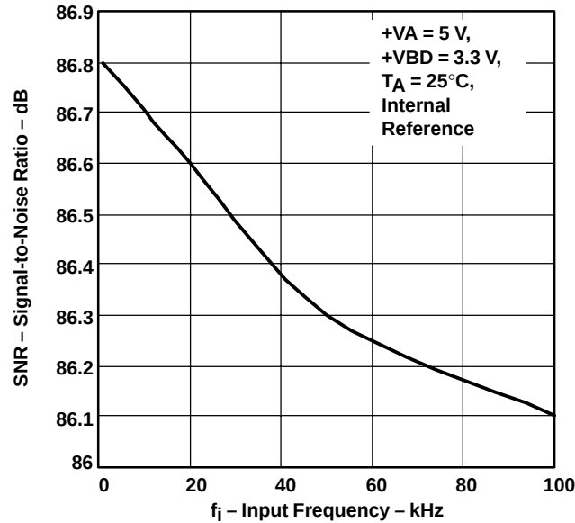
SIGNAL-TO-NOISE RATIO vs INPUT FREQUENCY
