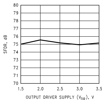
SFDR vs. DR \ V_D @ f_{IN} = 4.7 \text{ MHz}, f_{QIN} = 9.5 \text{ MHz}
