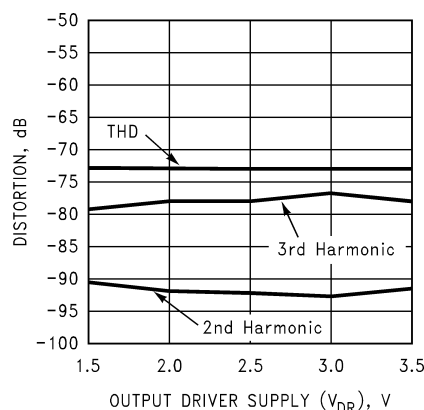
Distortion vs. DR \ V_D @ f_{IN} = 4.7 \text{ MHz}, f_{QIN} = 9.5 \text{ MHz}
