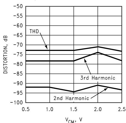
Distortion vs. V_{CM} @ f_{IN} = 4.7 \text{ MHz}, f_{QIN} = 9.5 \text{ MHz}
