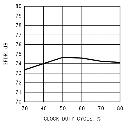
SFDR vs. Clock Duty Cycle @ f_{IN} = 4.7 \text{ MHz}
