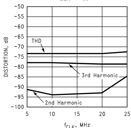
Distortion vs. f_{CLK} @ f_{IN} = 9.5 \text{ MHz}
