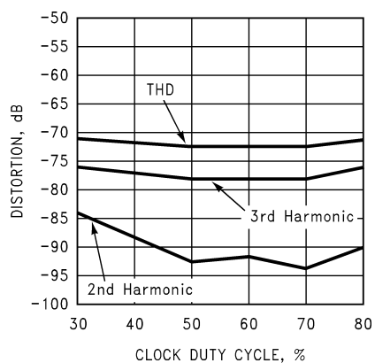
Distortion vs. Clock Duty Cycle @ f_{IN} = 4.7 \text{ MHz}
