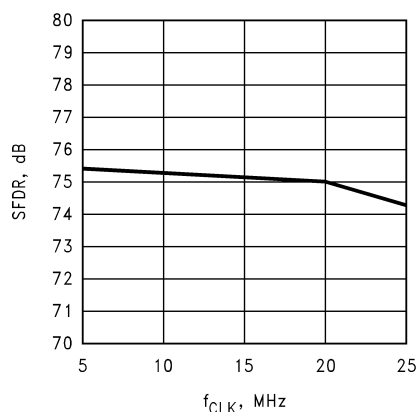
SFDR vs. f_{CLK} @ f_{IN} = 9.5 \text{ MHz}
