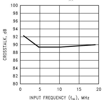
Crosstalk vs. f_{IN}
