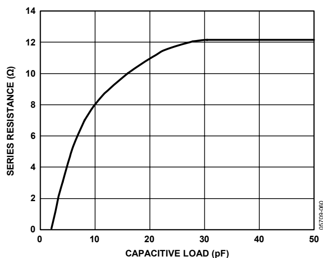
Figure 54. Recommended R_{\text{SERIES}} vs. Capacitive Load
