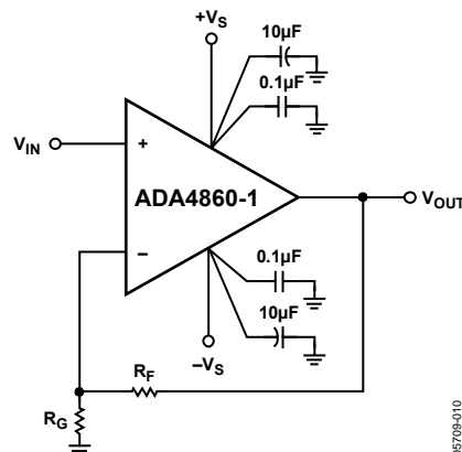
Figure 51. Noninverting Gain
