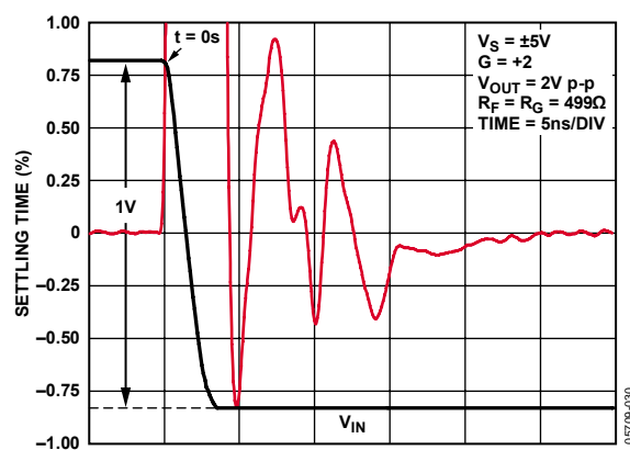
Figure 39. Settling Time Falling Edge
