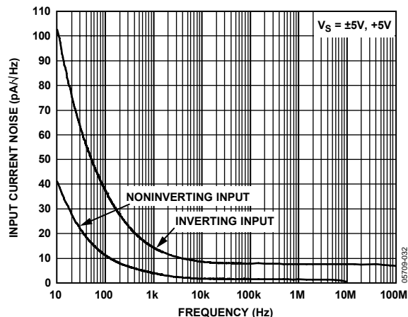
Figure 43. Input Current Noise vs. Frequency
