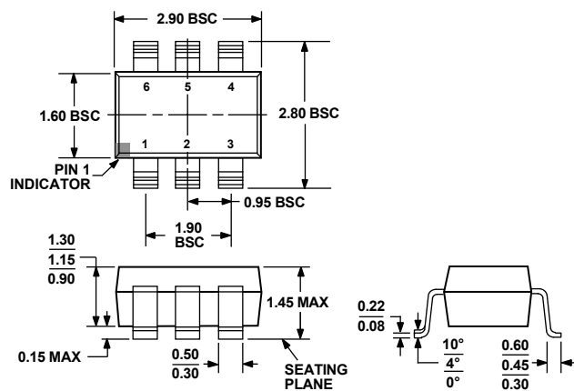
COMPLIANT TO JEDEC STANDARDS MO-178-AB Figure 62. 6-Lead Plastic Surface-Mount Package [SOT-23] (RJ-6) Dimensions shown in millimeters and (inches)
