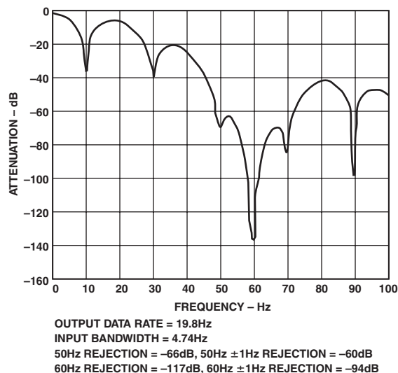
Figure 4. Filter Profile (Filter Notches at Both 50\text{ Hz} and 60\text{ Hz} )
