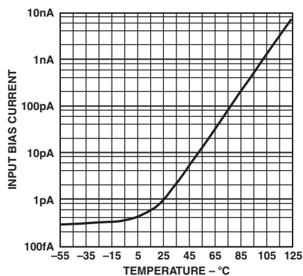
TPC 15. Pin 2 Input Bias Current vs. Temperature
