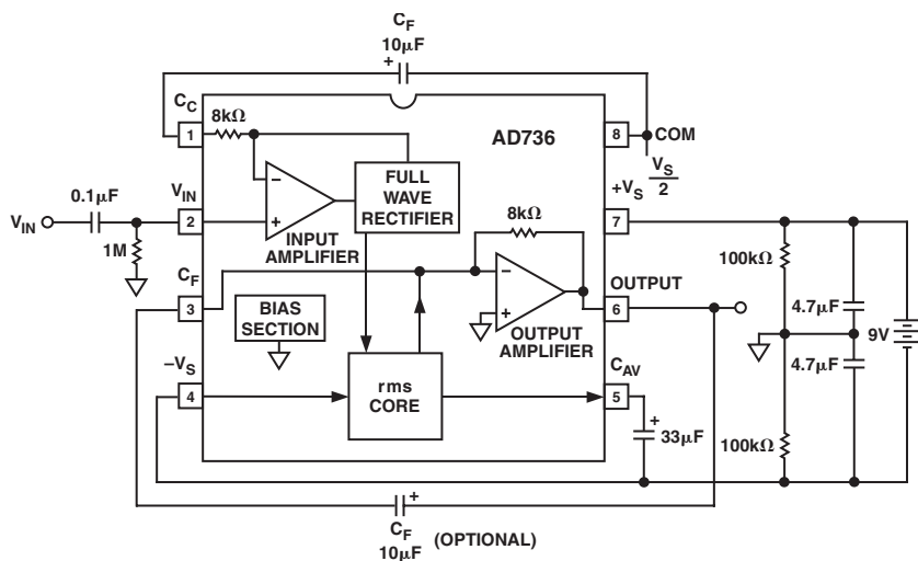
Figure 7. Battery-Powered Option
