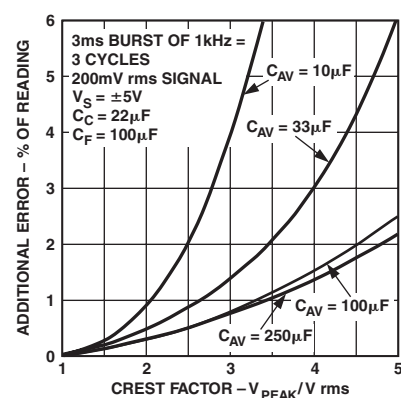
TPC 6. Additional Error vs. Crest Factor vs. C_{AV}
