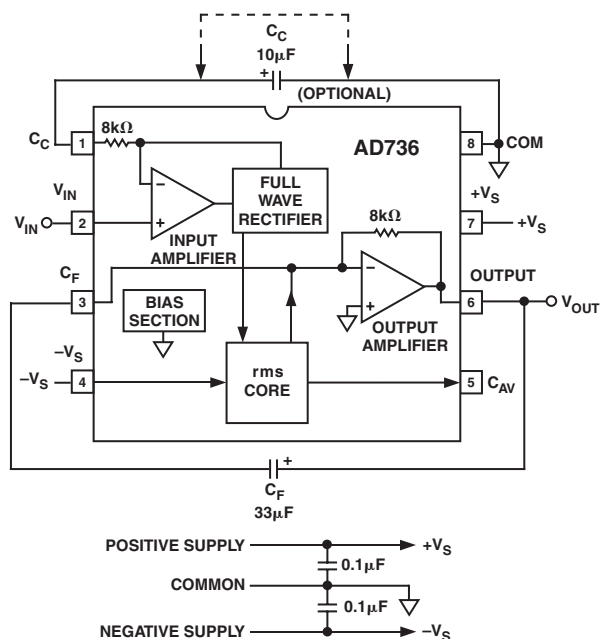
Figure 2. AD736 Average Responding Circuit
