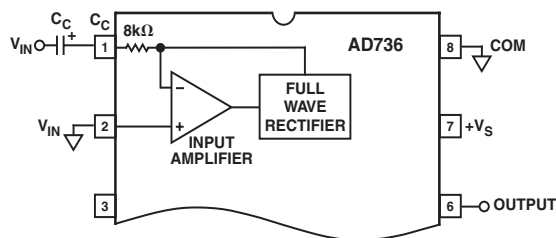
Figure 8. Low Z, AC-Coupled Input Connection
