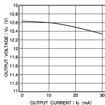
Fig. 7 Output characteristic
