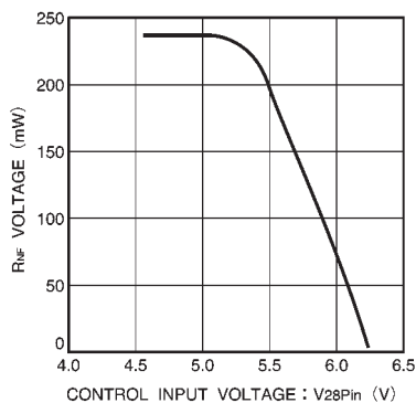
Fig.10 R_{DS} voltage vs. control input voltage
