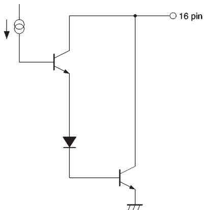
(6) Hall bias (16 pin)
