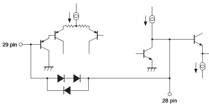
(8) Integrating amplifier (28, 29 pin)
