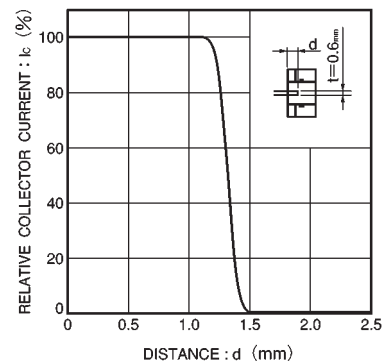
Fig.6 Relative output current vs. distance (1)
