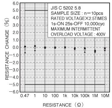
Fig.10 Intermittent overload
