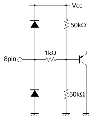
CPSEL
