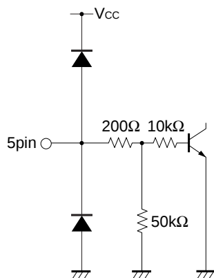
VSYNC IN
