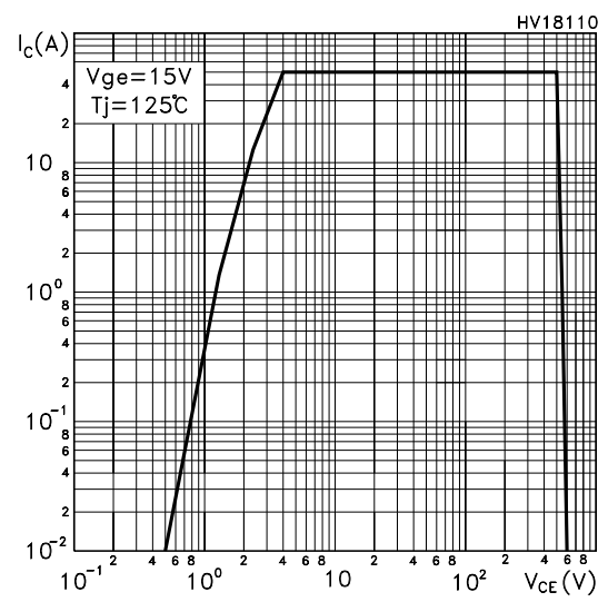
Turn-Off SOA
