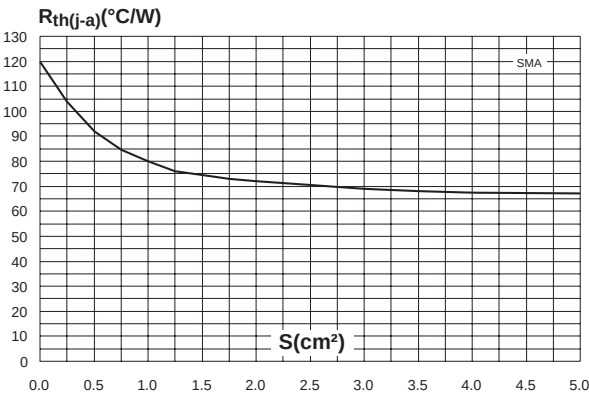
Fig. 10: Thermal resistance junction to ambient versus copper surface under each lead (Epoxy printed circuit board FR4, Cu: 35μm) (SMA).
