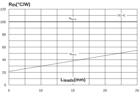
Fig. 11: Thermal resistance versus lead length (DO-15).
