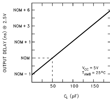
Figure 14. Typical Output Delay Variations versus Load Capacitance
