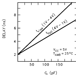
Figure 15. Typical Rise and Fall Variations versus Load Capacitance
