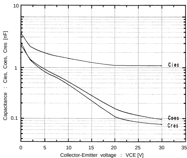
Capacitance vs. Collector-Emmitter voltage T_J=25^\circ C
