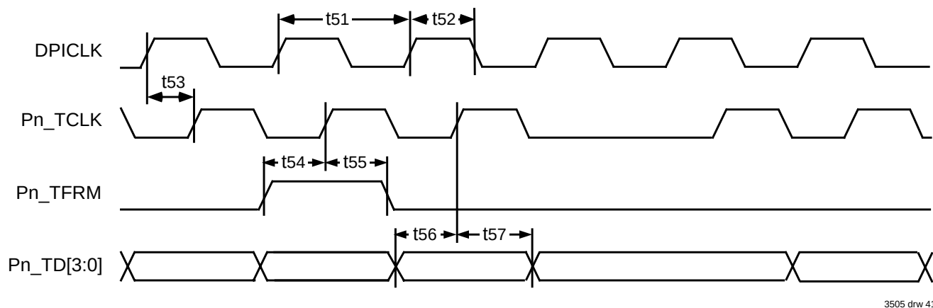
Figure 40. DPI Transmit
