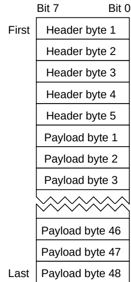
Figure 14. Utopia 1 Data Format and Sequence
