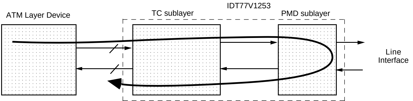
Figure 33. PHY Loopback
