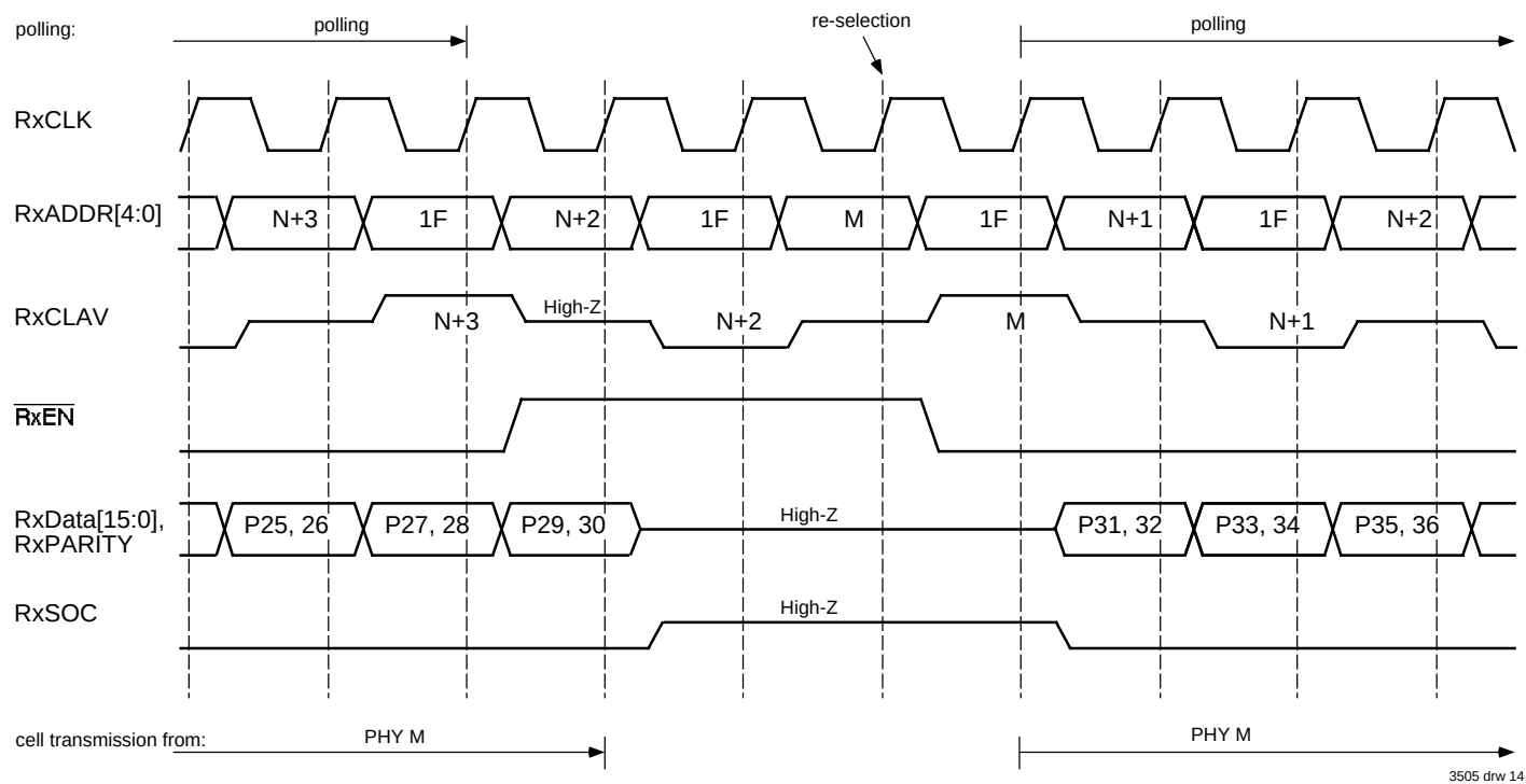
Figure 13. Utopia 2 Receive Handshake - Suspended Transfer of Data
