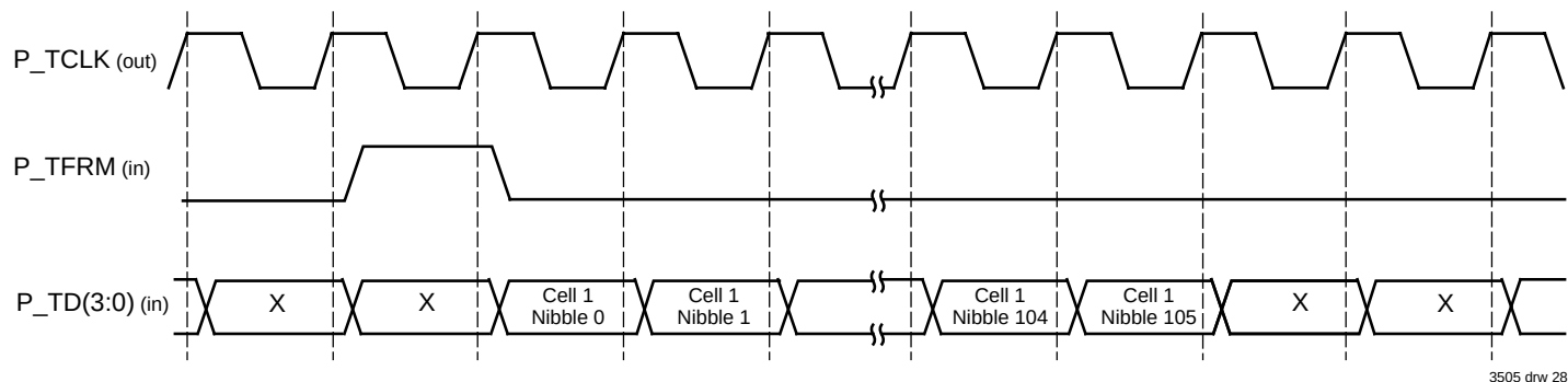
Figure 27. DPI Transmit Handshake - One Cell for Transmission
