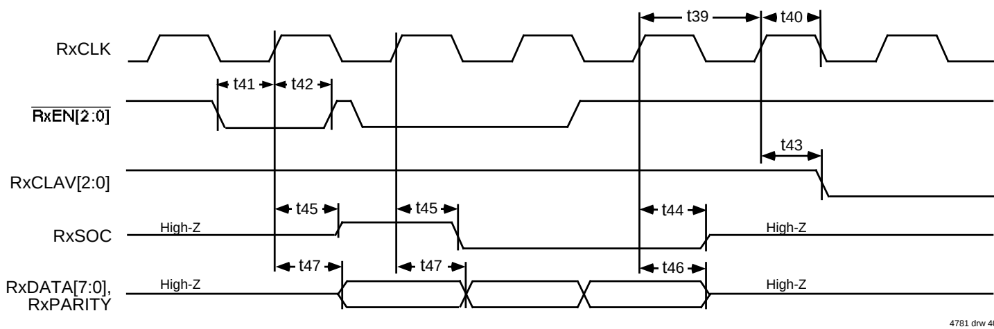
Figure 39. UTOPIA Level 1 Receive
