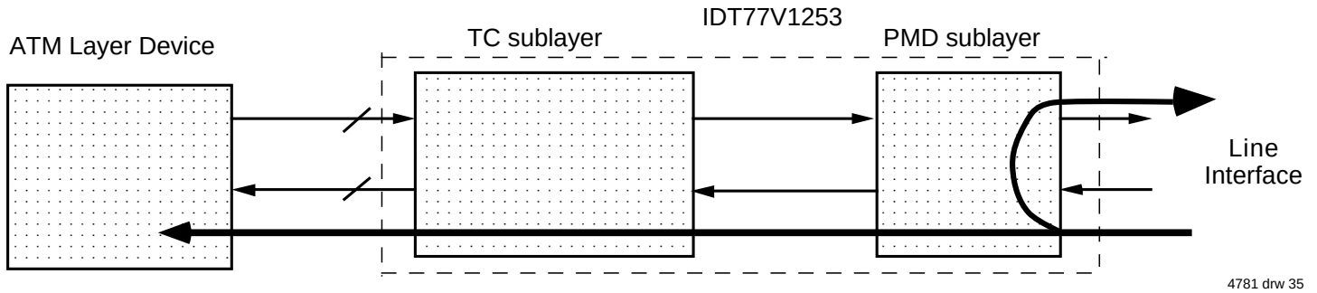
Figure 34. Line Loopback
