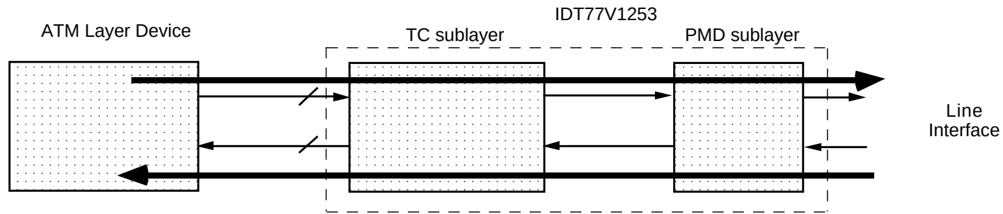
Figure 32. Normal Mode
