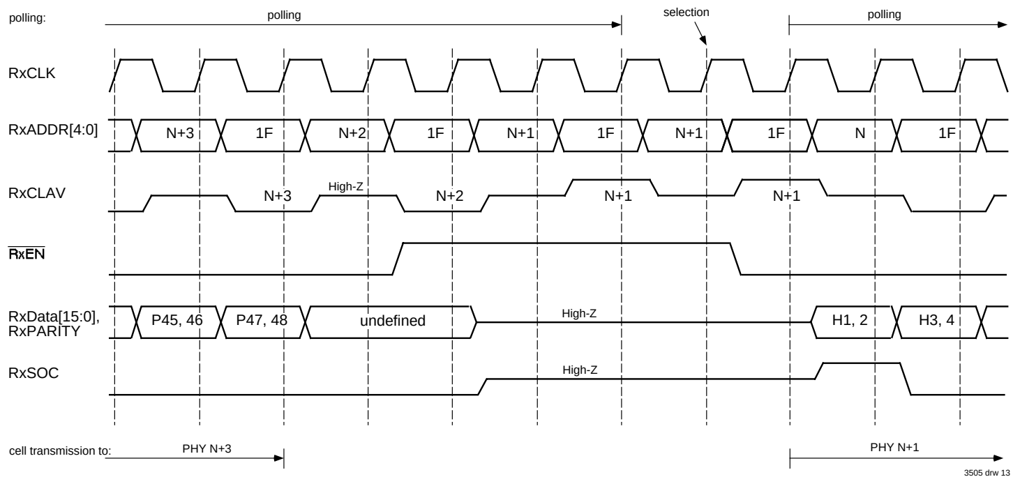
Figure 12. Utopia 2 Receive Handshake - Delay Between Cells
