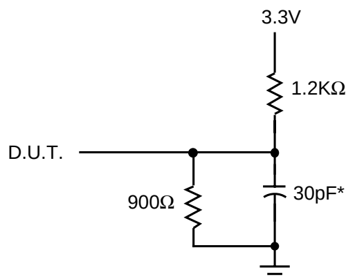
Figure 45. Output Load
