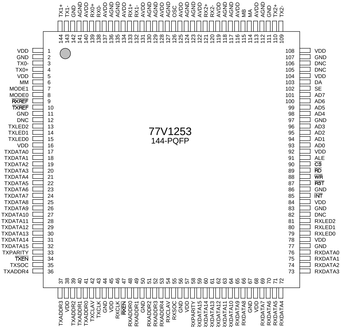
Figure 1. Pin Assignments
