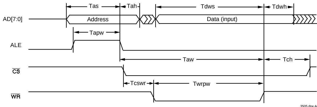
Figure 43. Utility Bus Write Cycle
