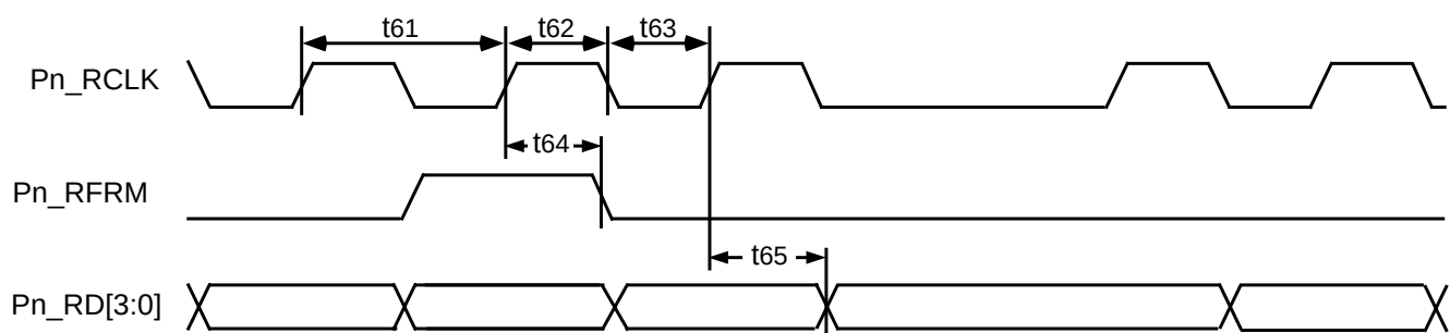
Figure 41. DPI Receive
