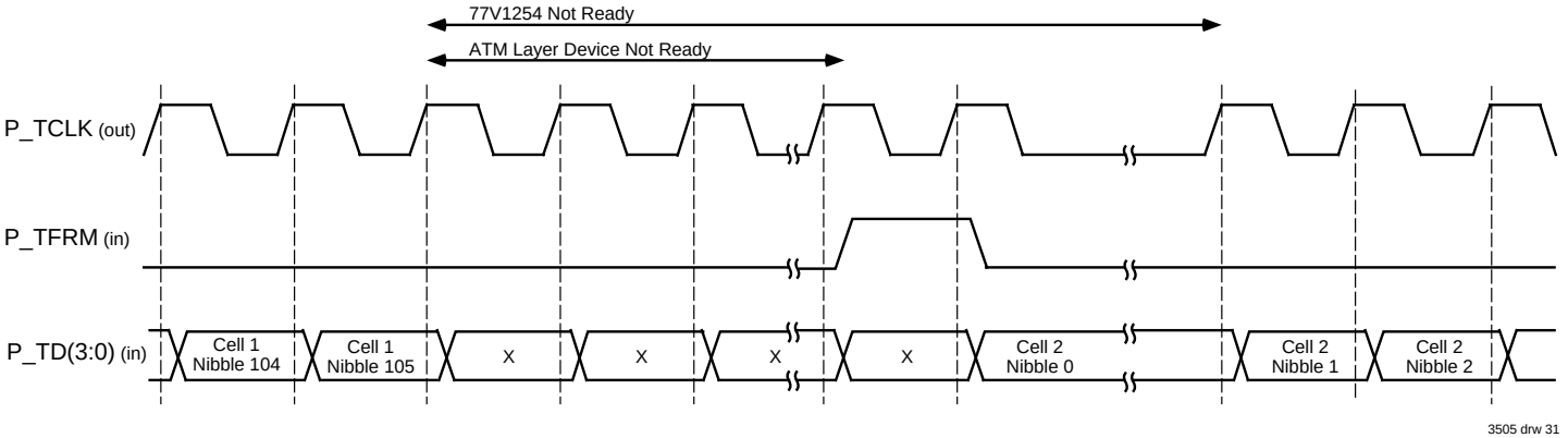
Figure 30. DPI Transmit Handshake - Neither Device Ready
