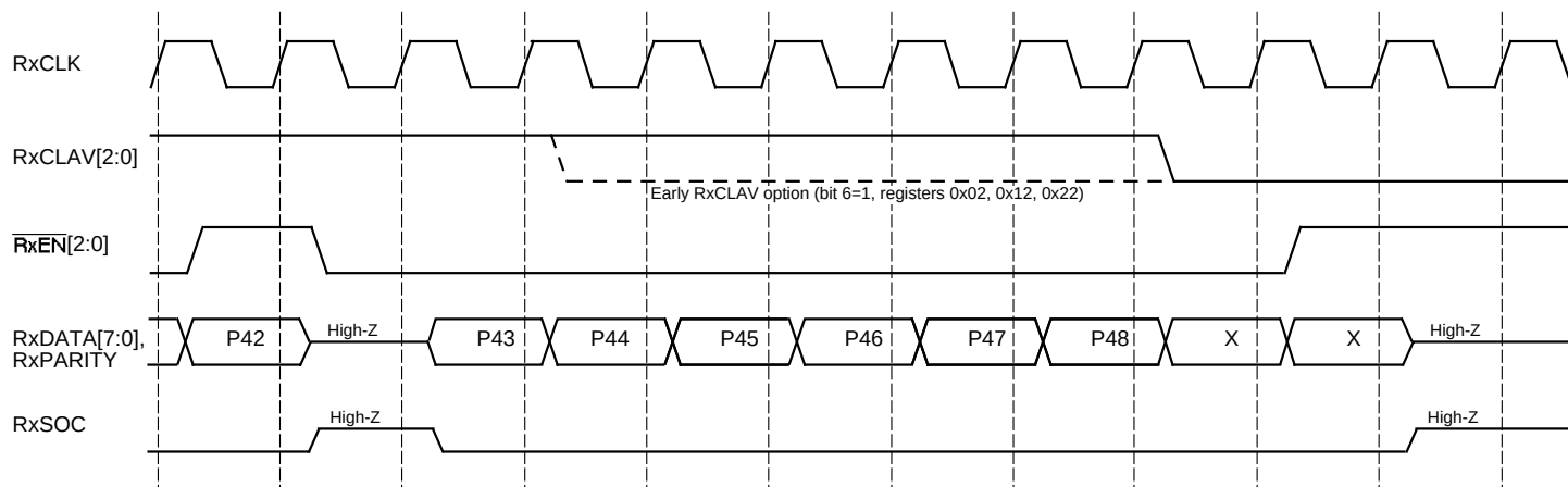
Figure 20. Utopia 1 Receive Handshake - RXCLAV Deassertion
