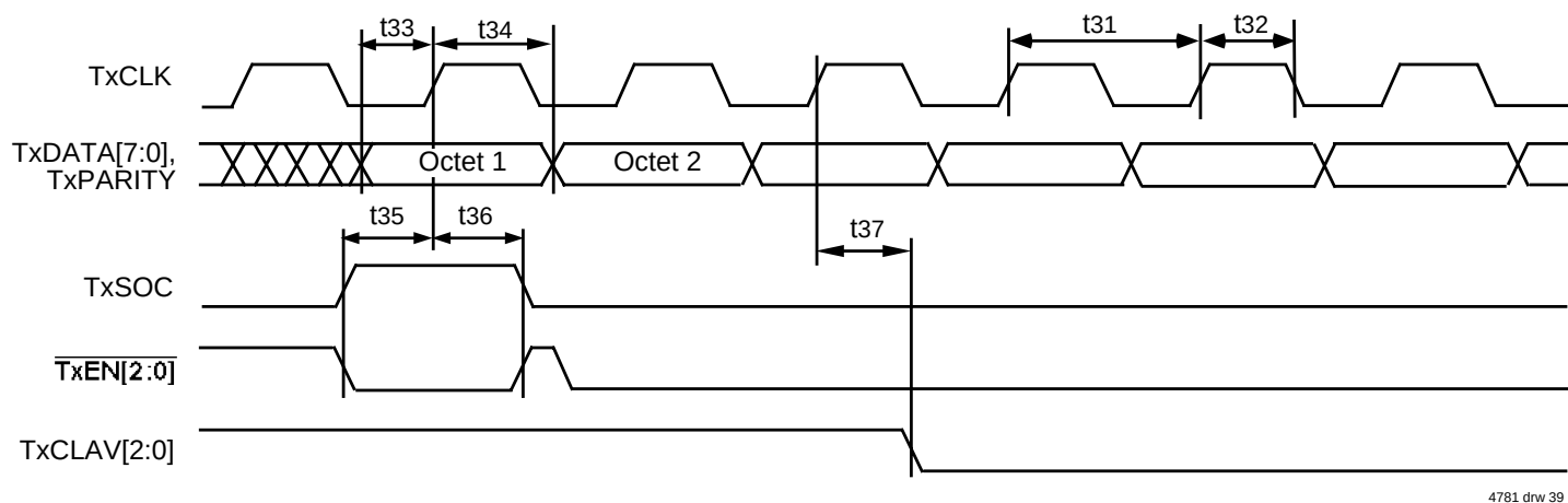
Figure 38. UTOPIA Level 1 Transmit
