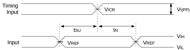
Voltage Waveforms - Setup and Hold Times
