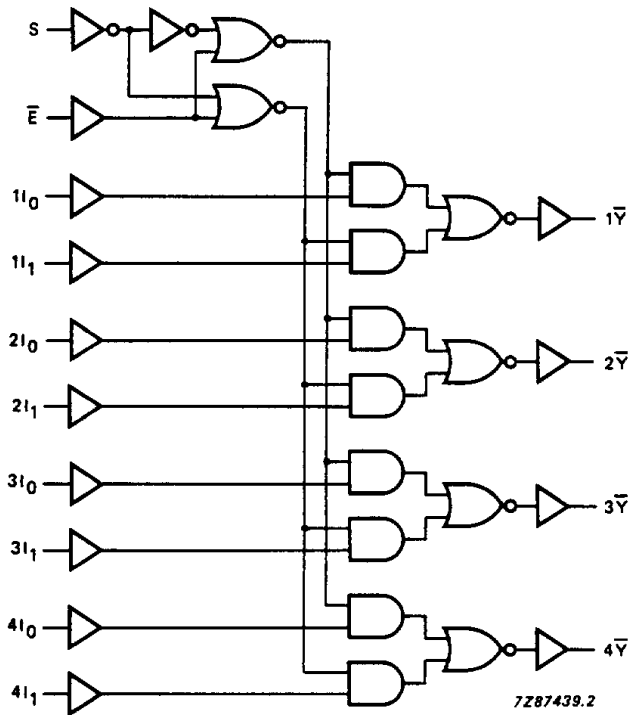
Fig.5 Logic diagram.
