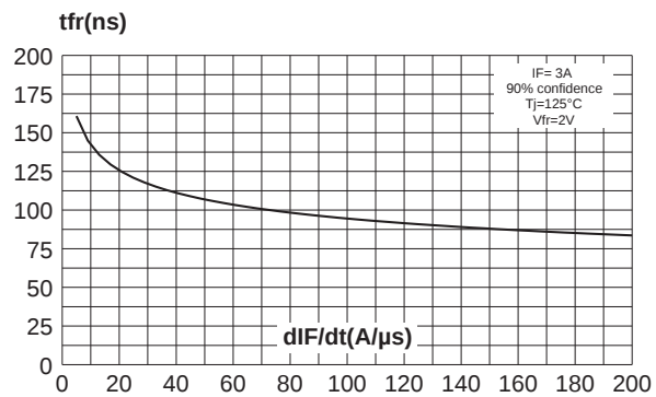
Fig. 9-2: Forward recovery time versus dI_F/dt (modulation diode).
