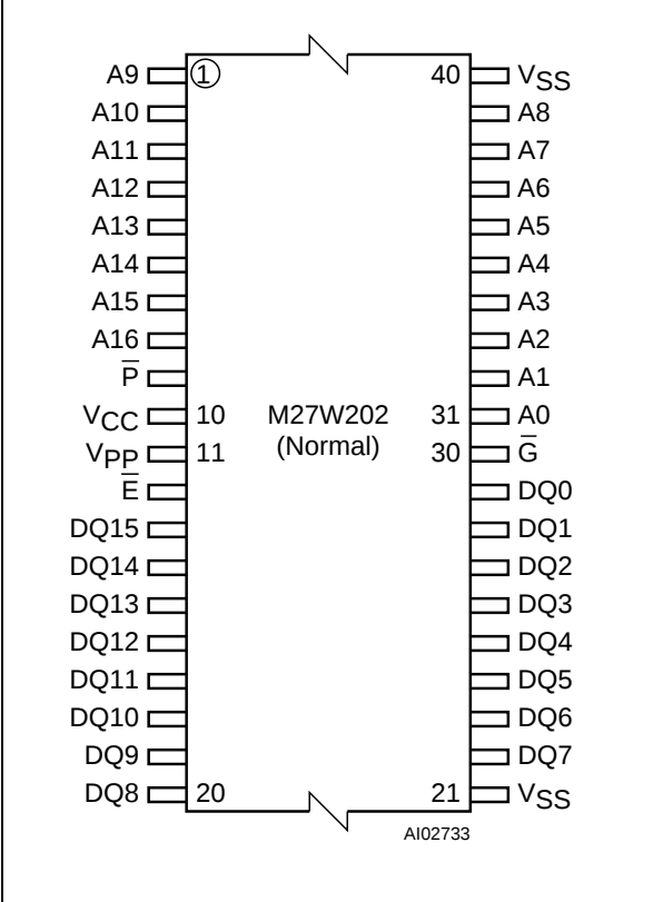
Figure 2C. TSOP Connections
