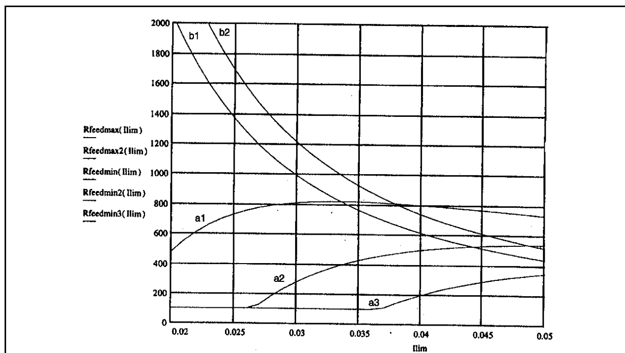
Figure B2. Rfeed allowed values vs. Ilim (Vbat = -54V).
