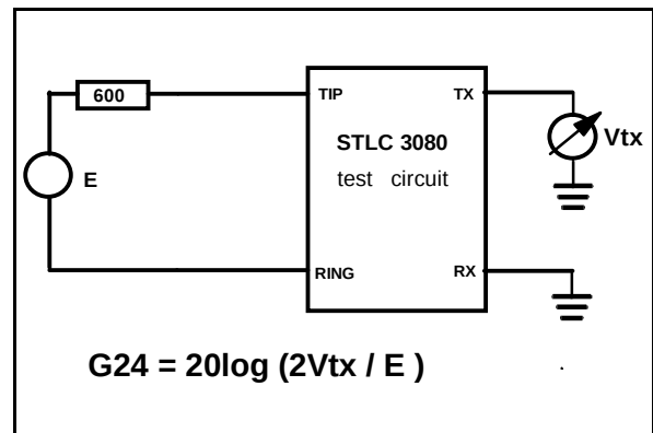
Figure C4. Transmit Gain.
