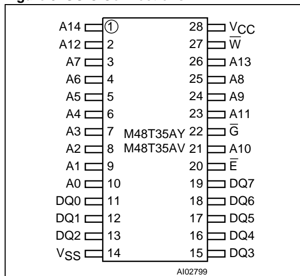
Figure 5. SOIC Connections
