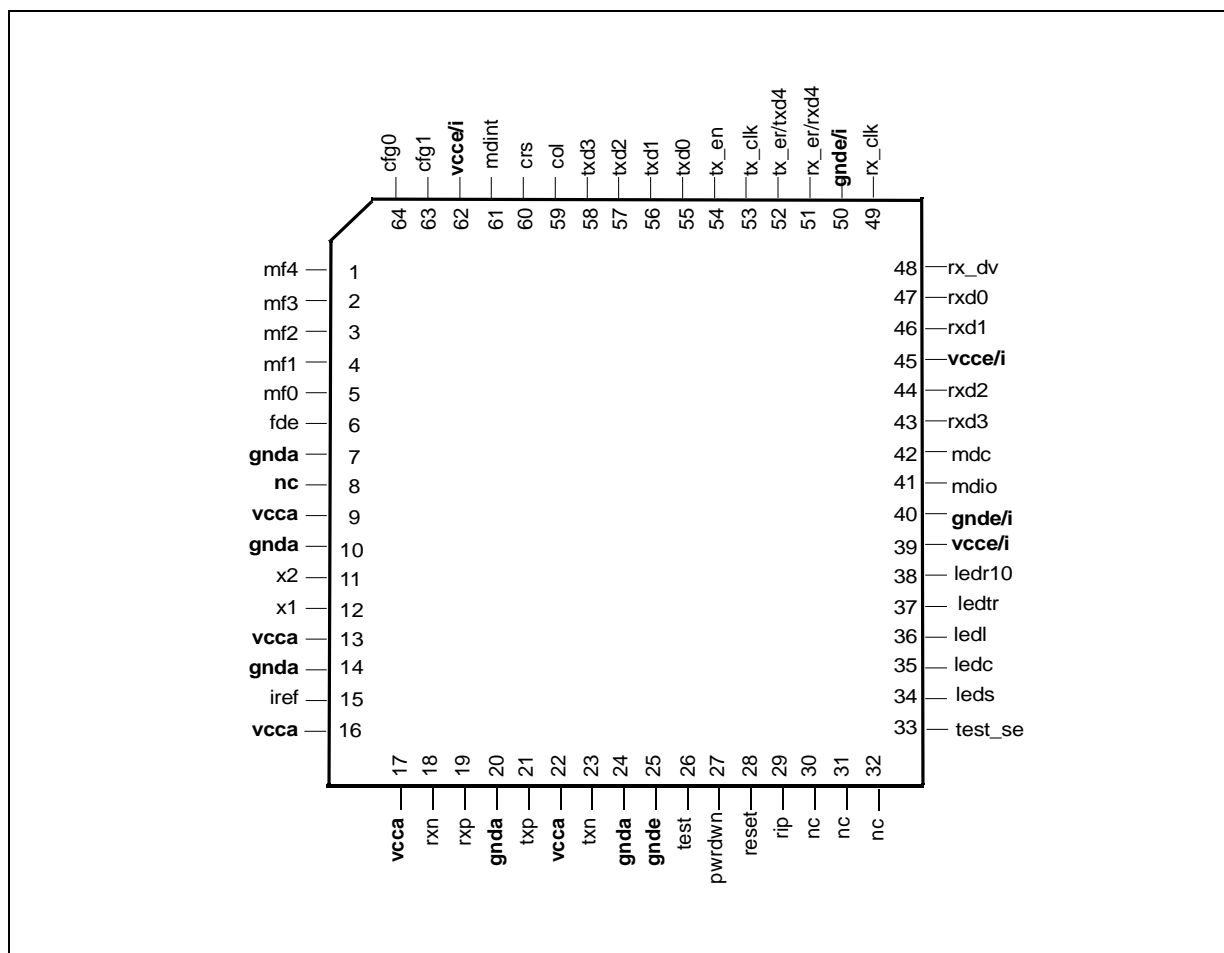
Figure 3. Pin Connection
