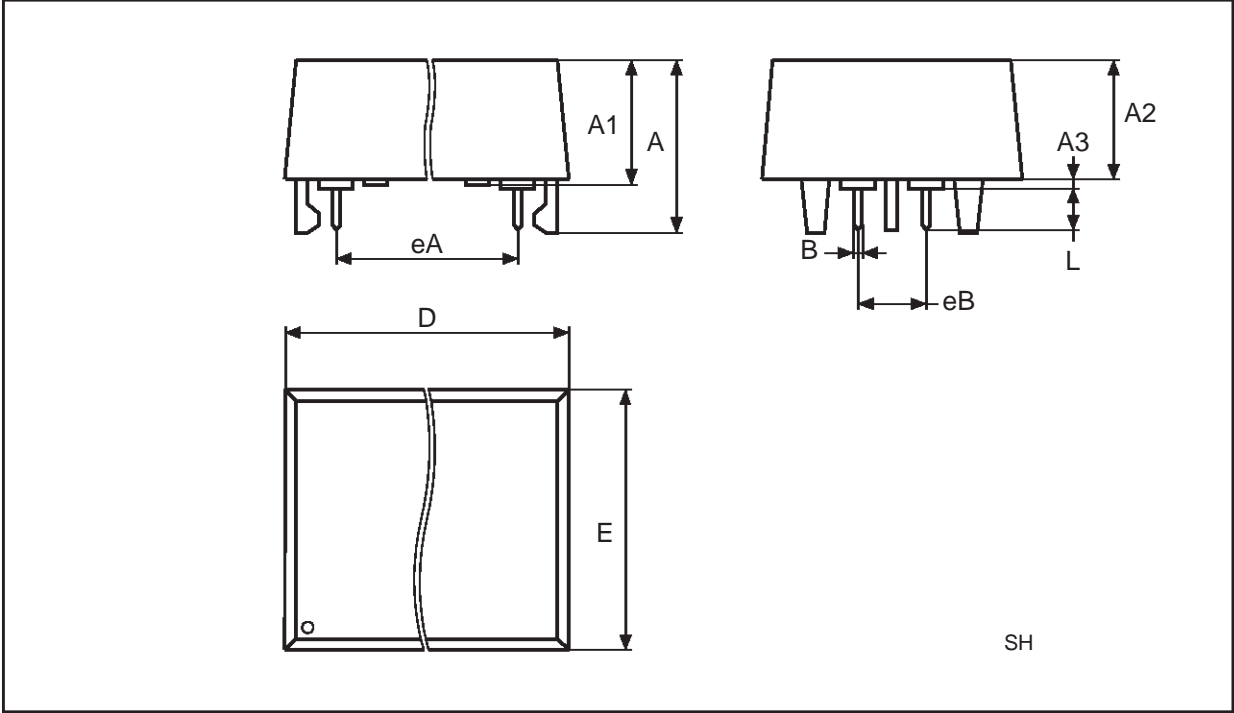
Figure 16. M4T32-BR12 - SNAPHAT Housing for 28 and 44 lead plastic SOIC, Package Outline
