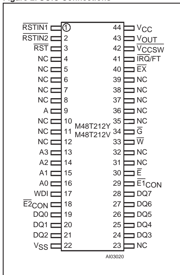
Figure 2. SOIC Connections
