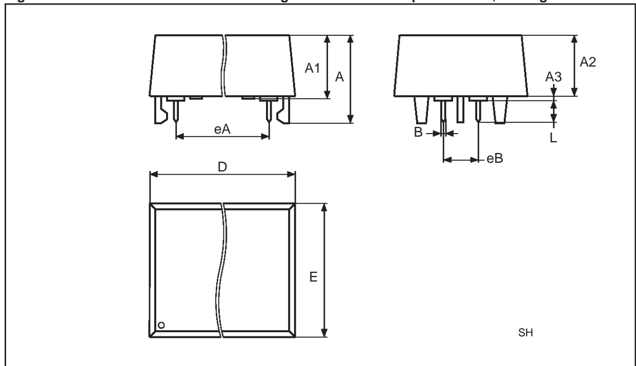
Figure 15. M4T28-BR12 - SNAPHAT Housing for 28 and 44 lead plastic SOIC, Package Outline
