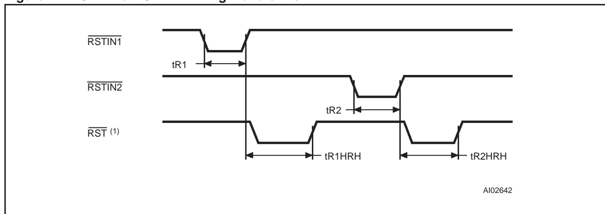
Figure 12. \overline{\text{RSTIN1}} & \overline{\text{RSTIN2}} Timing Waveforms
