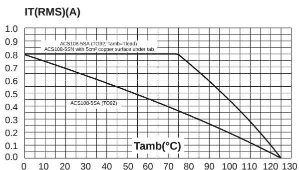
Fig. 6: RMS on-state current versus ambient temperature.
