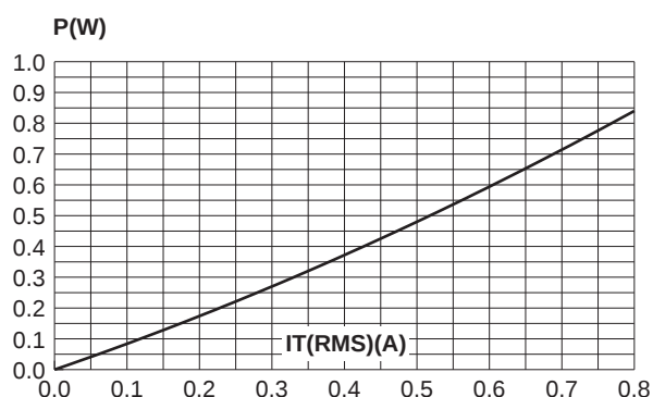
Fig. 5: Maximum power dissipation versus RMS on-state current.
