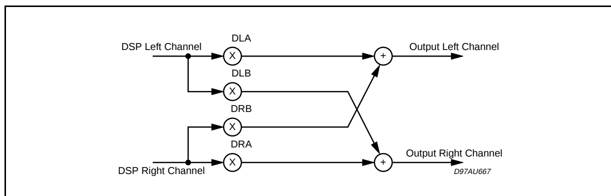
Figure 12. Volume Control and Output Setup
