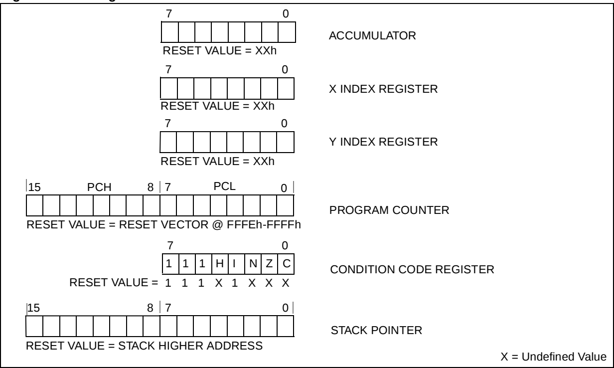
Figure 6. CPU Registers
