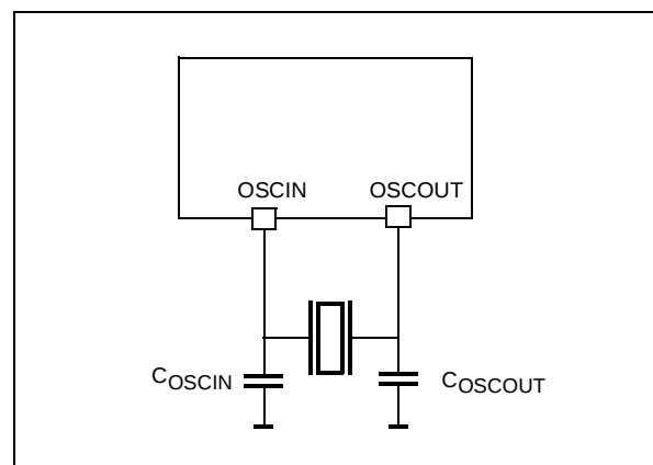
Figure 9. Crystal/Ceramic Resonator
