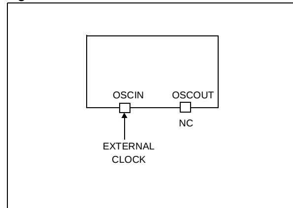
Figure 8. External Clock Source Connections
