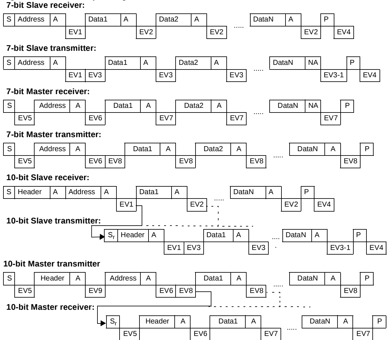
Figure 31. Transfer Sequencing
